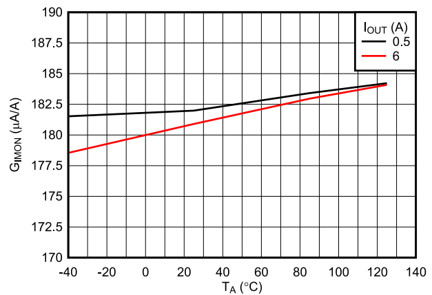
Figure 6-19. Analog Current Monitor gain vs Temperature
