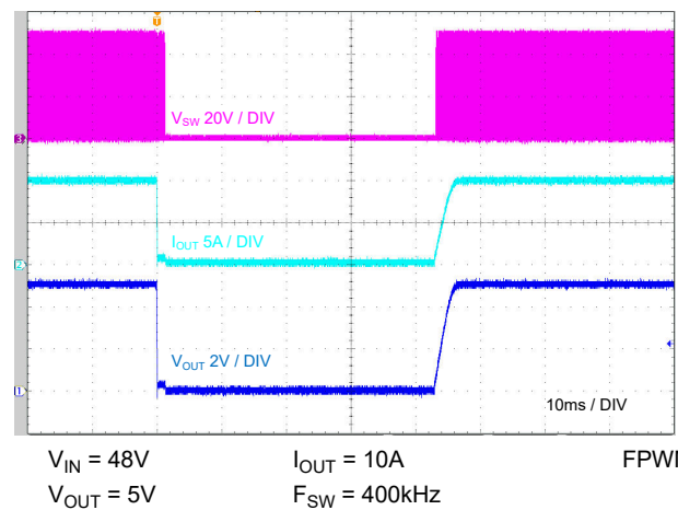
Figure 5-11. Short-Circuit Recovery
