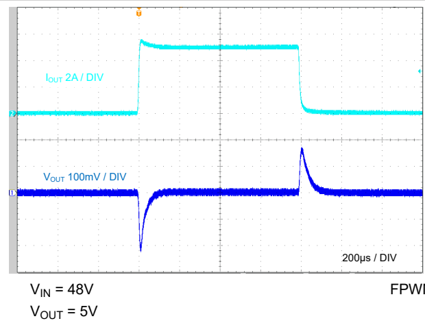
Figure 5-9. Load Transient, 0A to 5A
