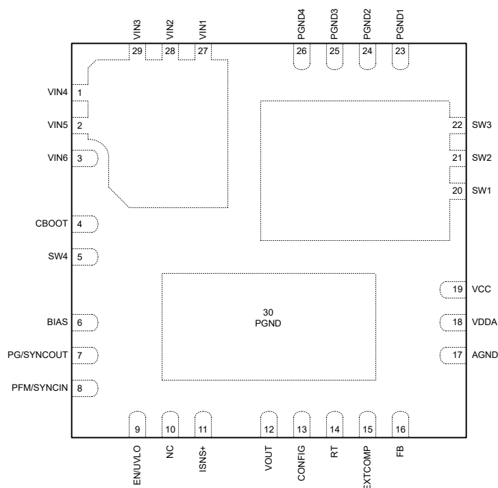
Figure 4-1. RRX Package, 29-Pin VQFN (Top View)
