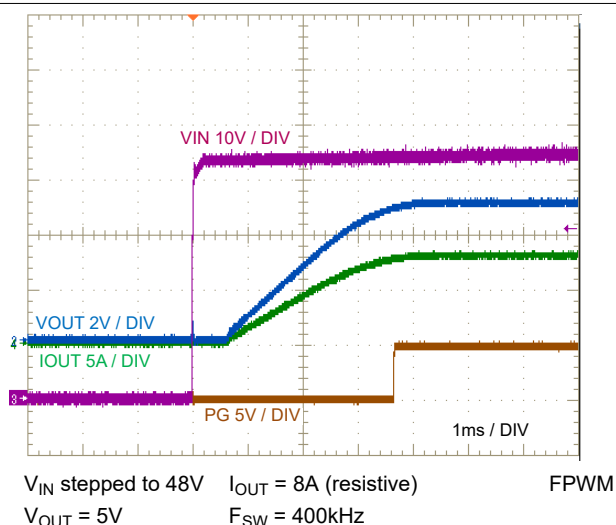
Figure 7-17. Start-Up Characteristic
