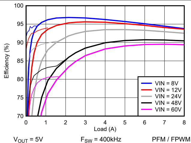
Figure 7-13. Efficiency versus I_{OUT}
