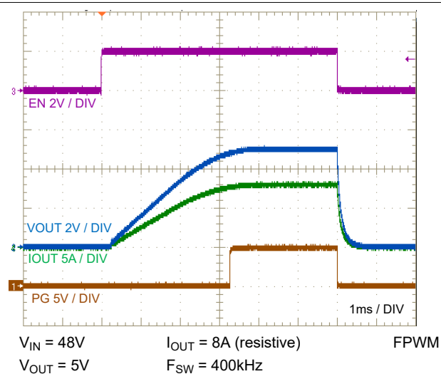
Figure 7-18. EN Start-Up Characteristic
