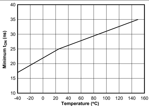
Figure 5-14. Minimum On-Time vs Temperature
