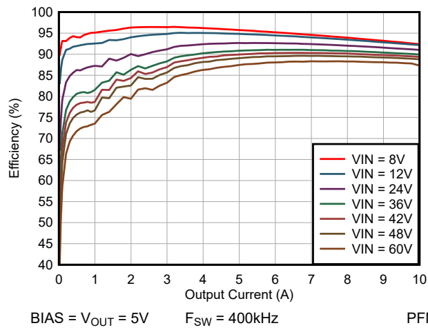
Figure 5-7. Efficiency vs I_{OUT} , Linear Scale
