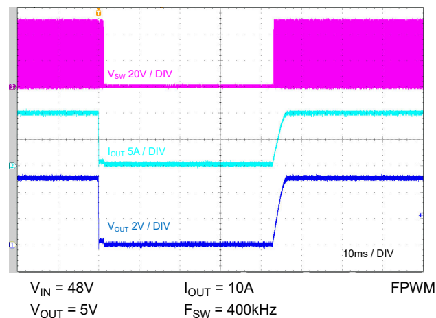
Figure 5-11. Short-Circuit Recovery
