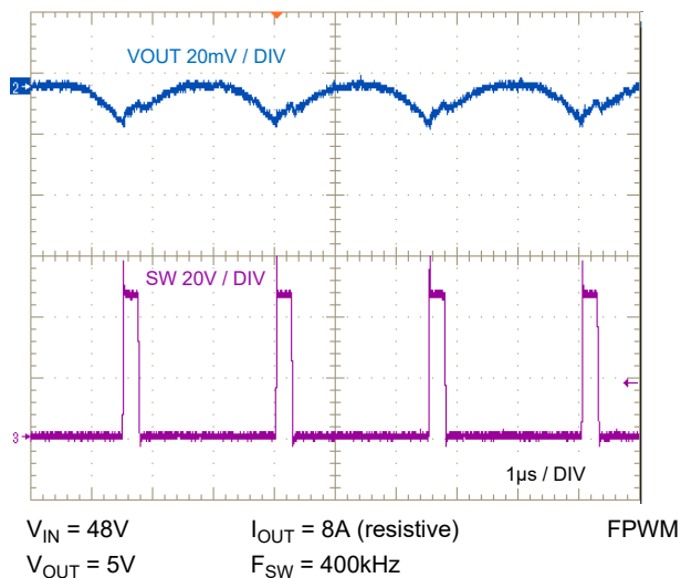
Figure 7-15. Full Load Switching
