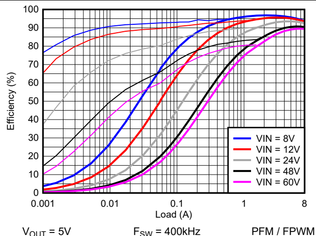
Figure 7-14. Efficiency versus I_{OUT} , Log Scale
