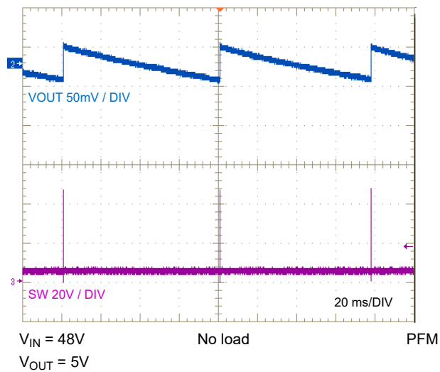
Figure 7-16. PFM Switching
