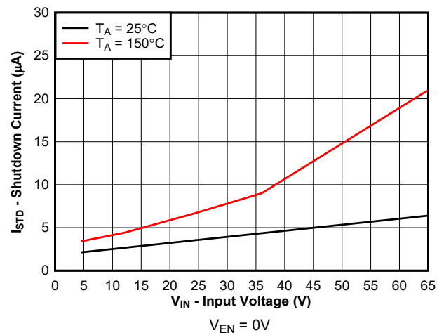
Figure 5-12. Shutdown Current vs Input Voltage
