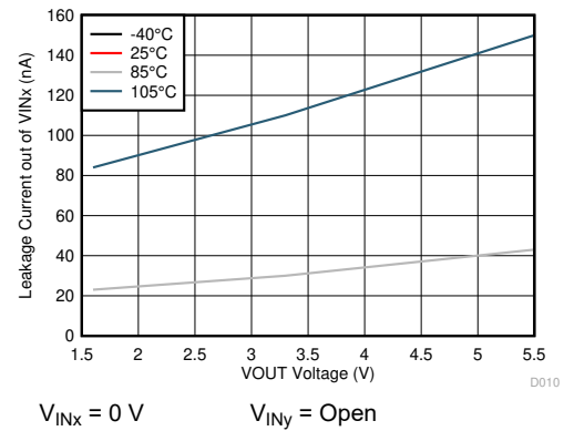
Figure 6-8. Reverse Leakage Current out of VINx
