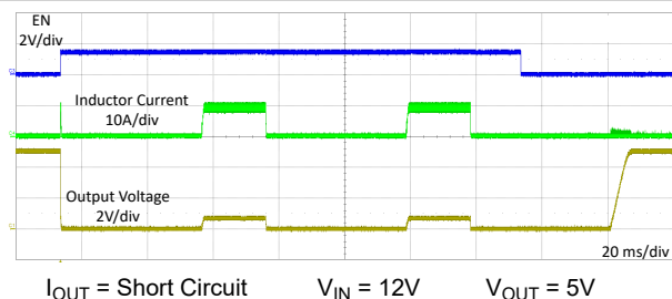
Figure 8-12. Short Circuit
