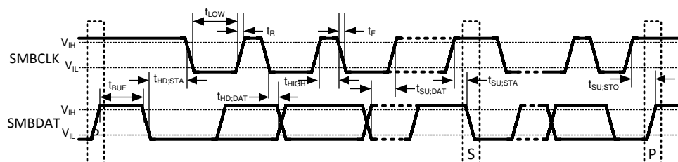
Figure 5-1. SMBus Timing Diagram for SMBCLK and SMBDAT Signals
