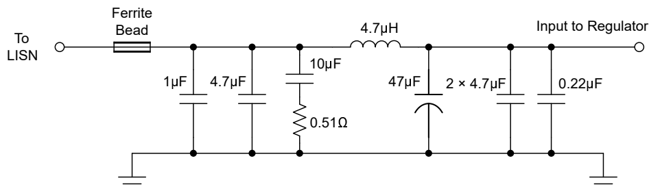
A. Input filter used only for EMI measurements shown in EMI Performance Curves .
