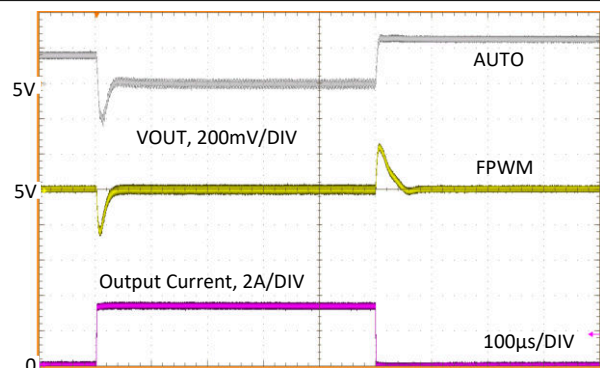
Figure 8-20. Load Transient
