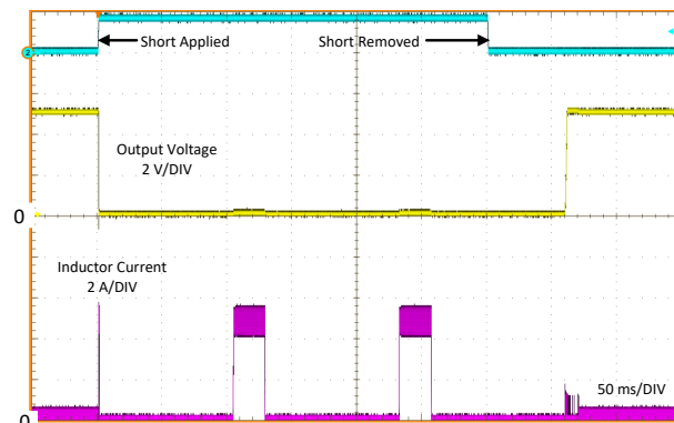
Figure 7-13. Short-Circuit Transient and Recovery
