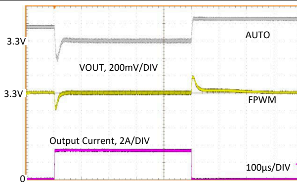
Figure 8-21. Load Transient
