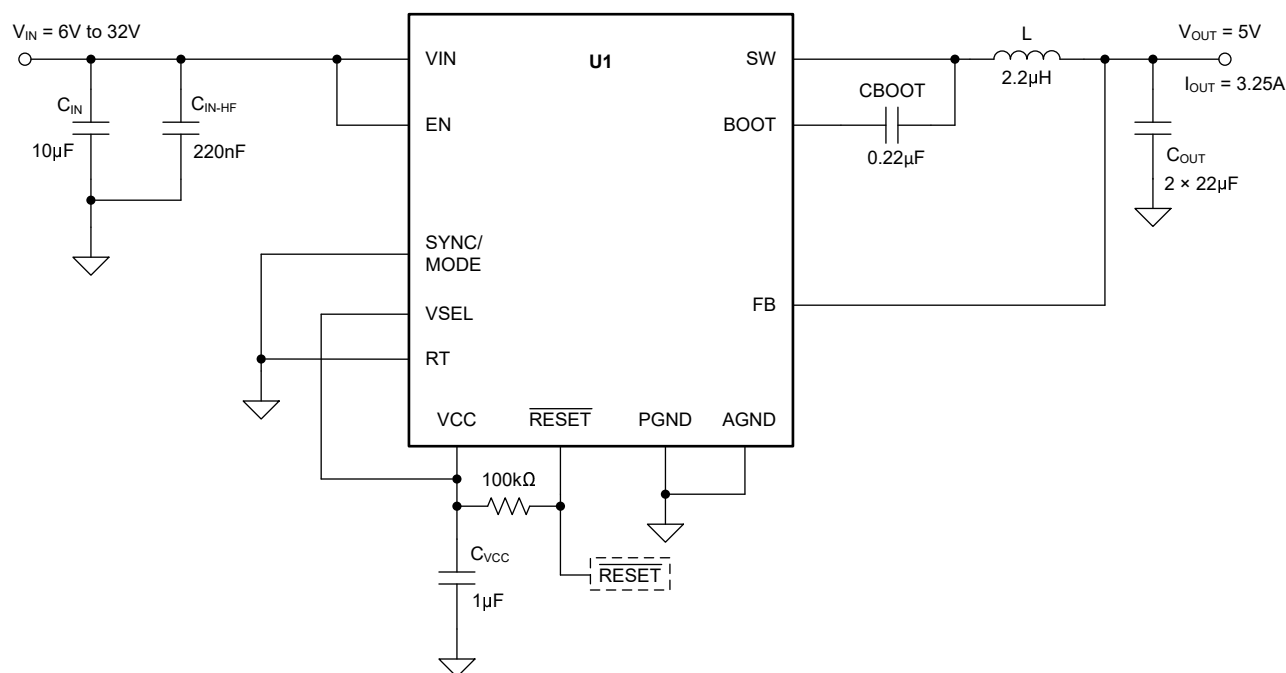
Figure 8-1. Example Application Circuit V_{IN} = 12\text{ V} , V_{OUT} = 5\text{ V} , I_{OUT} = 3.25\text{ A} , f_{SW} = 2.1\text{ MHz}
