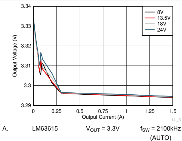
Figure 8-19. Line and Load Regulation
