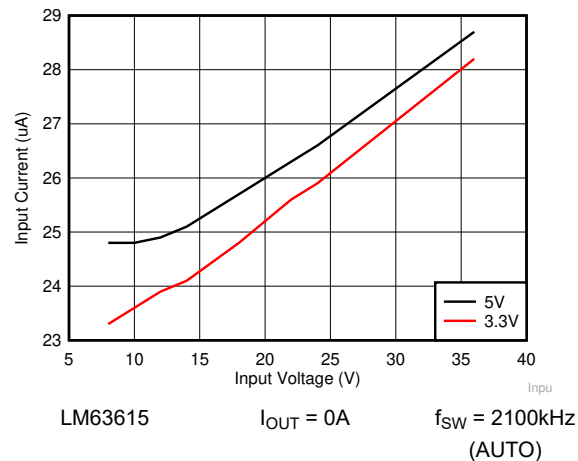
Figure 8-39. Input Supply Current versus Input Voltage
