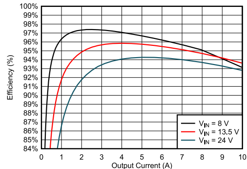
EVM Efficiency with \theta_{JA} = 21.6^\circ\text{C/W} : V_{OUT} = 5\text{ V} , F_{SW} = 0.4\text{ MHz}
