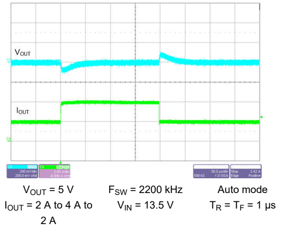
Figure 9-44. Load Transient
