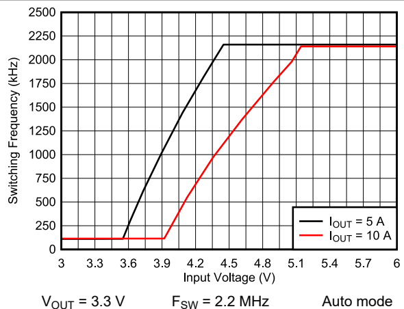
Figure 9-28. Frequency Dropout
