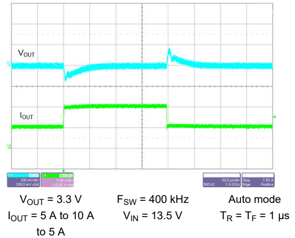
Figure 9-42. Load Transient
