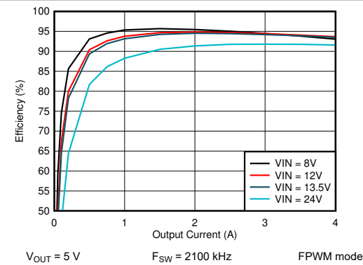
Figure 10-8. LM62440-Q1 Efficiency
