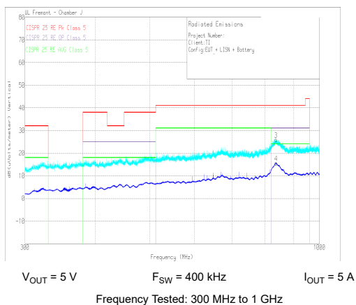
Figure 10-31. Radiated EMI Log Vertical versus CISPR25 Limits, LM61460EVM
