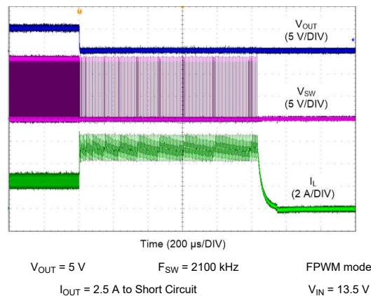
Figure 10-20. LM62440-Q1 Short Circuit Protection
