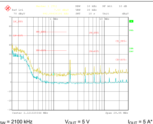
Figure 10-32. Radiated EMI Log Horizontal versus CISPR25 Limits, LM61460EVM
