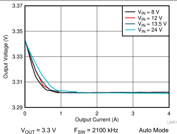
Figure 10-9. LM62440-Q1 Load and Line Regulation
