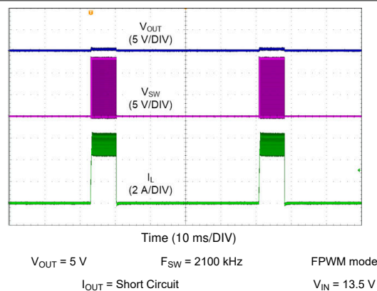
Figure 10-22. LM62440-Q1 Short Circuit Performance
