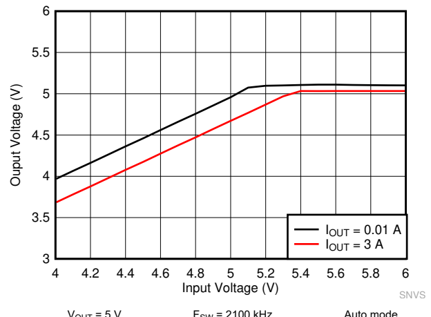
Figure 10-14. LM62440-Q1 Dropout Curve
