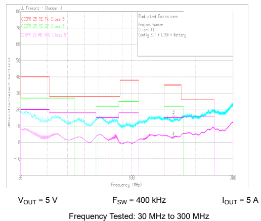
Figure 10-30. Radiated EMI Bicon Horizontal versus CISPR25 Limits, LM61460EVM
