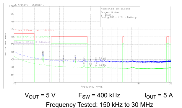
Figure 10-28. Radiated EMI Rod versus CISPR25 Limits, LM61460EVM
