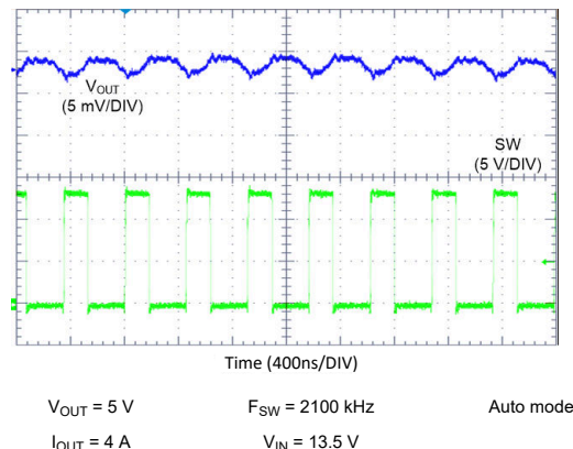
Figure 10-18. LM62440-Q1 Switching Waveform and V_{OUT} Ripple
