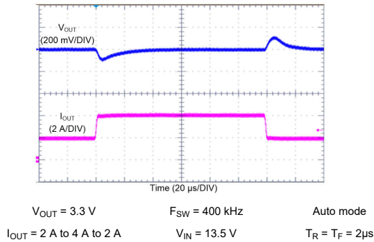
Figure 10-23. LM62440-Q1 Load Transient
