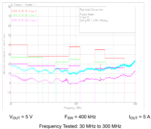
Figure 10-29. Radiated EMI Bicon Vertical versus CISPR25 Limits, LM61460EVM
