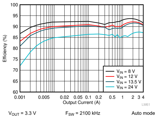
Figure 10-5. LM62440-Q1 Efficiency
