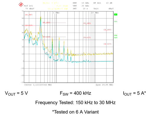
Figure 10-26. Conducted EMI versus CISPR25 Limits (Yellow: Peak Signal, Blue: Average Signal), LM61460EVM
