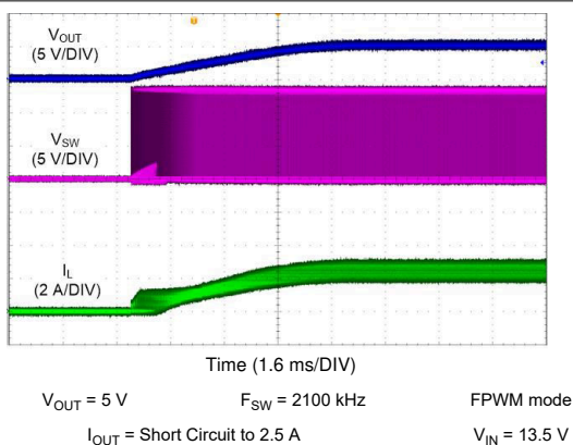
Figure 10-21. LM62440-Q1 Short Circuit Recovery
