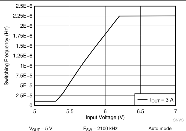
Figure 10-16. LM62440-Q1 Frequency Dropout Curve
