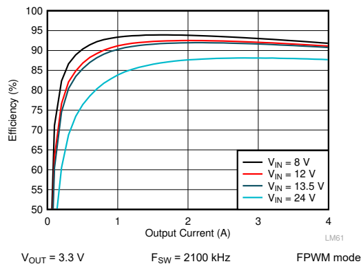
Figure 10-6. LM62440-Q1 Efficiency
