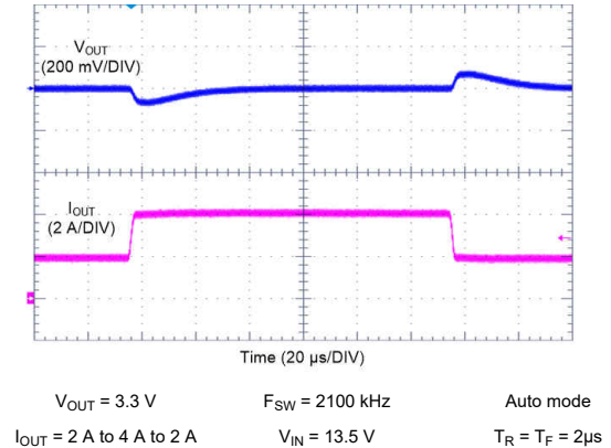
Figure 10-24. LM62440-Q1 Load Transient
