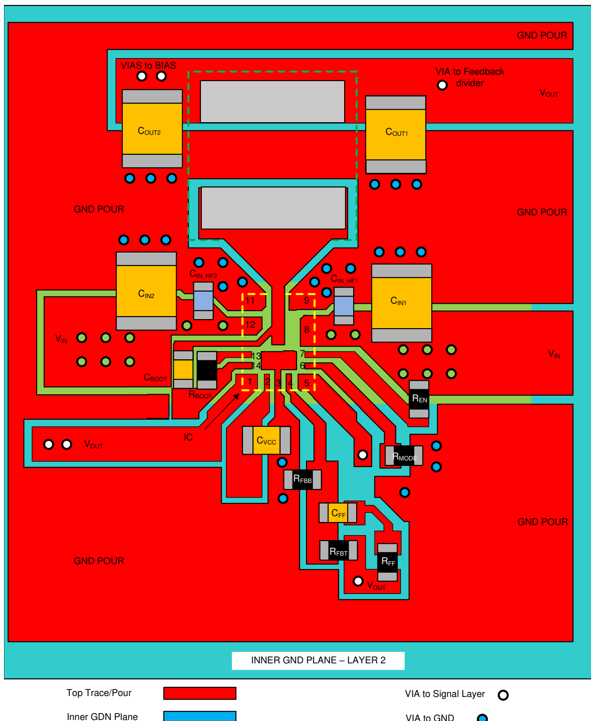
Figure 12-2. Layout Example
