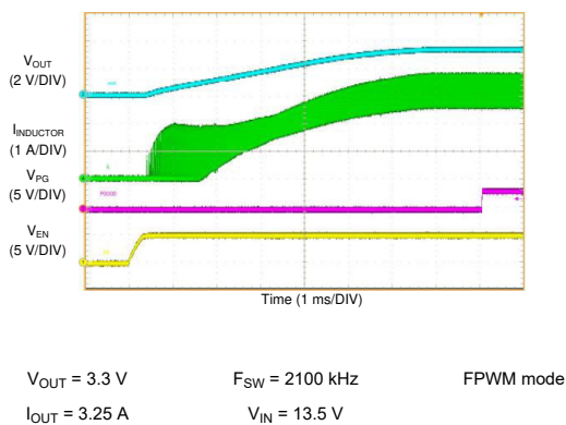
Figure 10-19. LM62440-Q1 Start-up with 3.25-A
