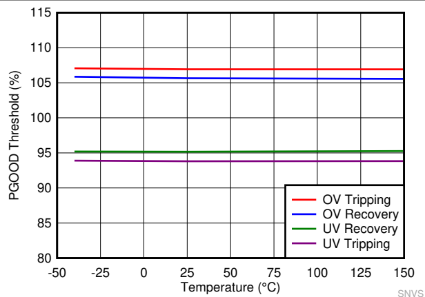
Figure 8-8. PGOOD Thresholds
