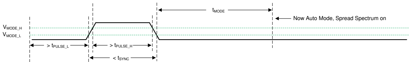
Figure 9-10. Transition from SYNC Mode to Auto Mode
