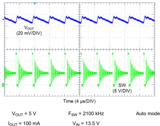
Figure 10-17. LM62440-Q1 Switching Waveform and V_{OUT} Ripple
