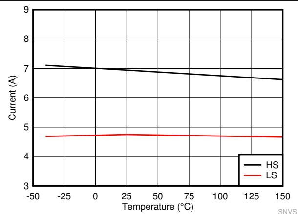
Figure 8-4. LM62440-Q1 High-Side and Low-Side Current Limits
