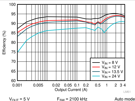
Figure 10-7. LM62440-Q1 Efficiency
