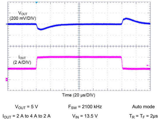
Figure 10-25. LM62440-Q1 Load Transient
