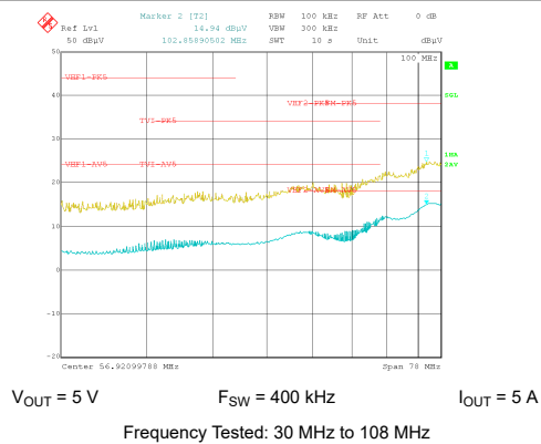
Figure 10-27. Conducted EMI versus CISPR25 Limits (Yellow: Peak Signal, Blue: Average Signal), LM61460EVM
