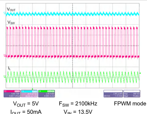
Figure 8-28. Switching Waveform and V_{OUT} Ripple
