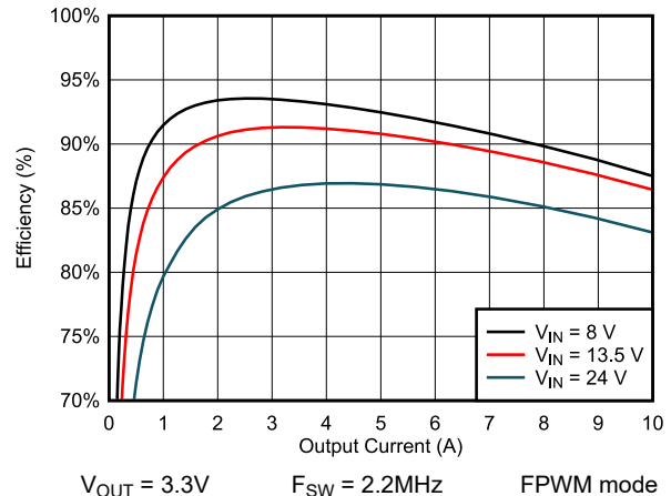
Figure 8-10. Efficiency
