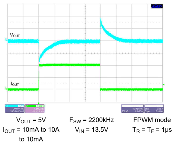
Figure 8-41. Load Transient
