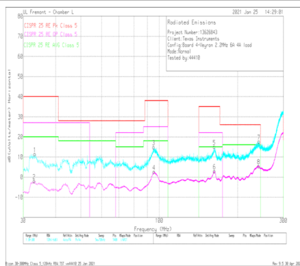
Figure 8-51. Radiated EMI Bicon Horizontal vs CISPR25 Class 5 Limits
