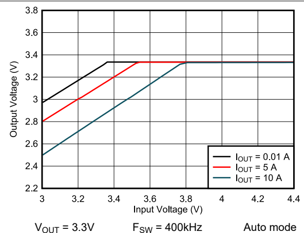
Figure 8-20. Dropout
