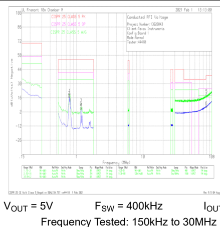
Figure 8-44. Conducted EMI versus CISPR25 Class 5 Limits (Green: Peak Signal, Blue: Average Signal)
