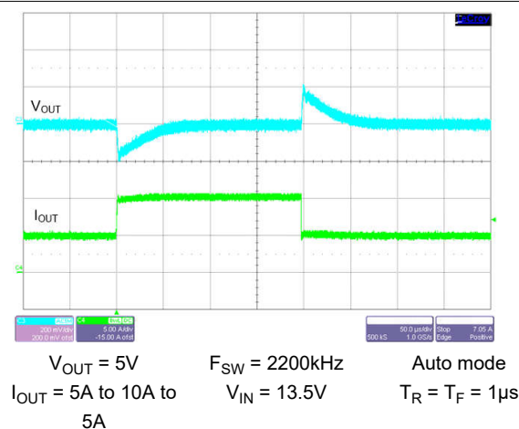
Figure 8-43. Load Transient
