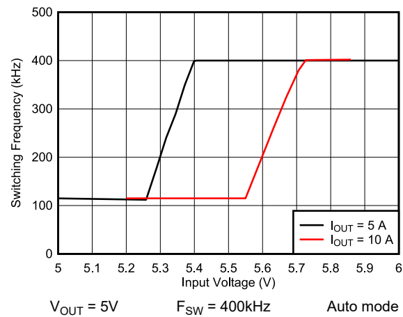
Figure 8-23. Frequency Dropout
