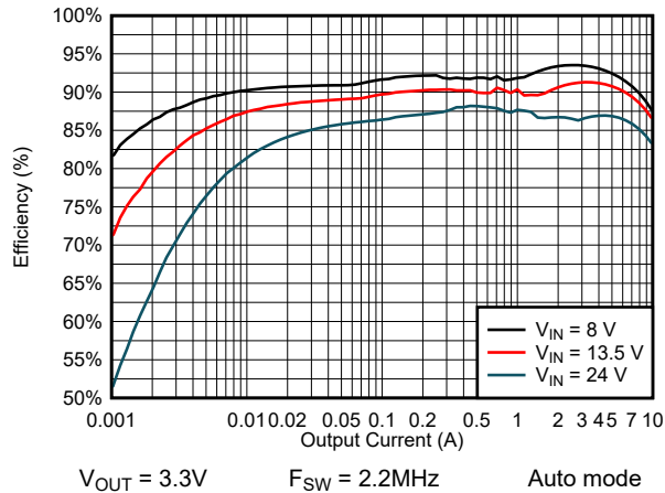
Figure 8-9. Efficiency
