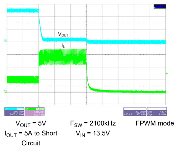
Figure 8-32. Short-Circuit Protection
