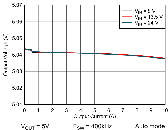
Figure 8-11. Load and Line Regulation
