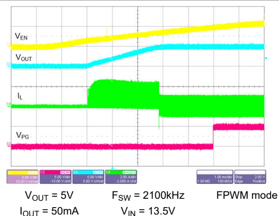
Figure 8-30. Start-Up With 50mA Load
