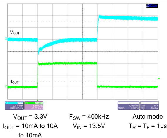
Figure 8-39. Load Transient
