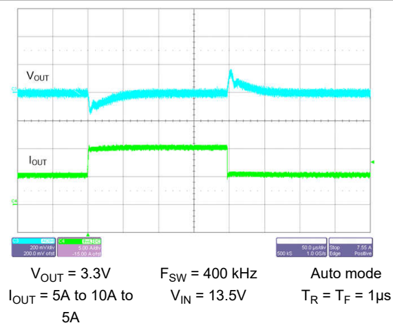
Figure 8-40. Load Transient
