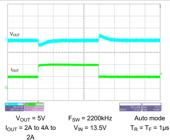
Figure 8-42. Load Transient
