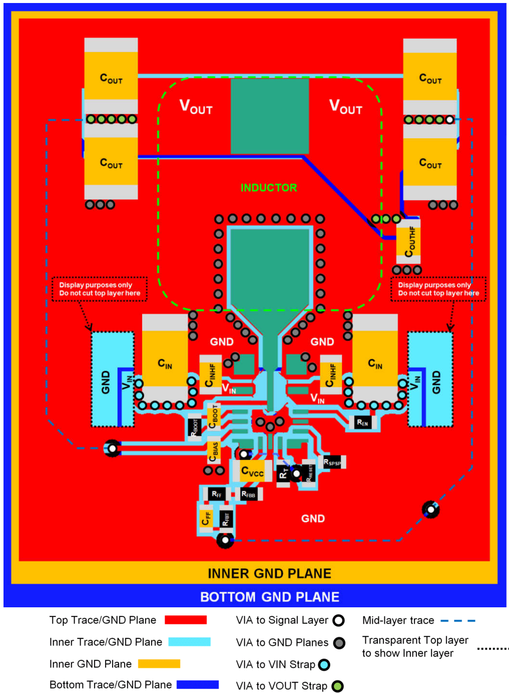
Figure 8-57. Layout Example
