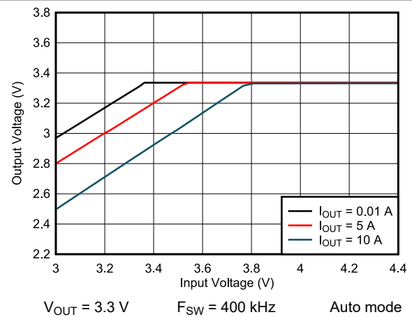
Figure 9-22. Dropout
