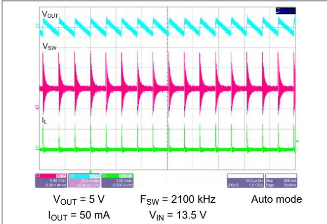
Figure 8-29. Switching Waveform and V_{OUT} Ripple
