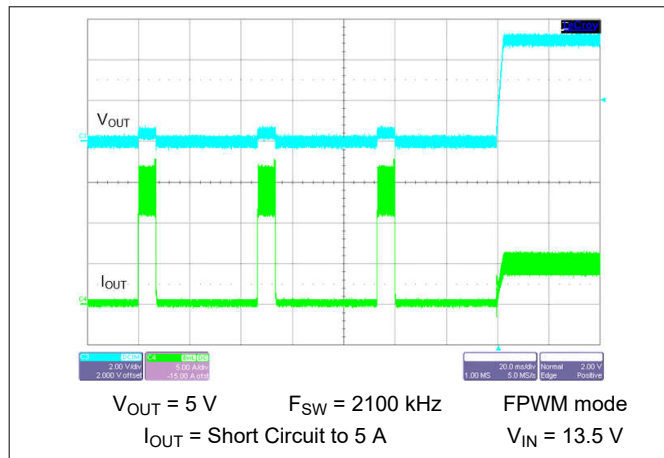
Figure 8-35. Short Circuit Recovery
