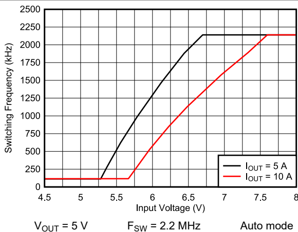
Figure 8-27. Frequency Dropout
