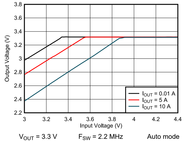
Figure 8-24. Dropout
