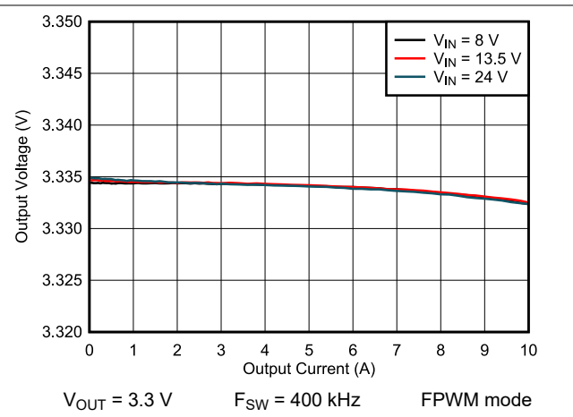
Figure 8-16. Load and Line Regulation
