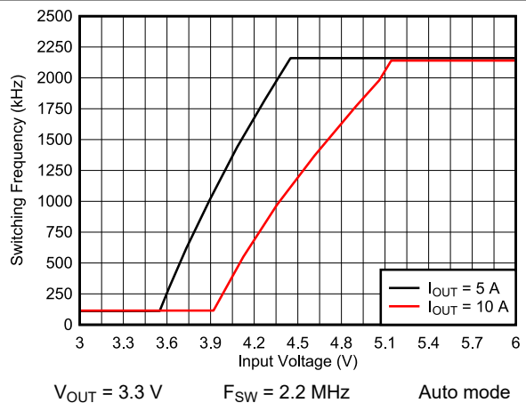
Figure 8-28. Frequency Dropout
