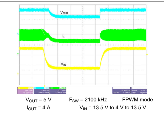
Figure 8-36. Recovery from Dropout
