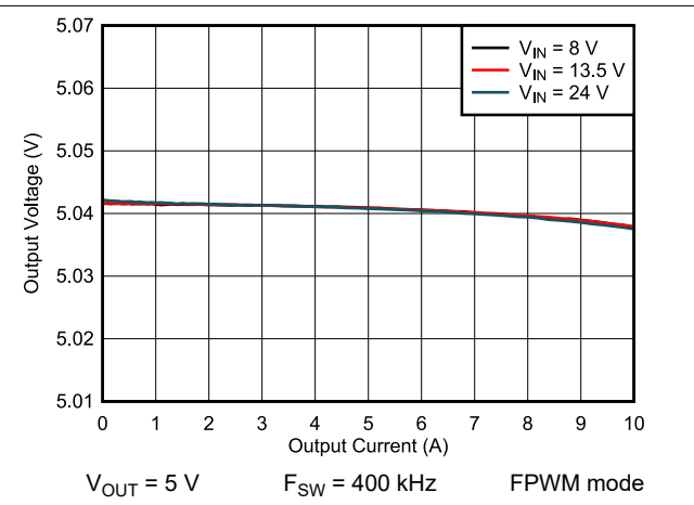
Figure 8-14. Load and Line Regulation
