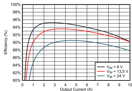
EVM Efficiency: V_{OUT} = 5\text{V} , F_{SW} = 2.2\text{MHz}
