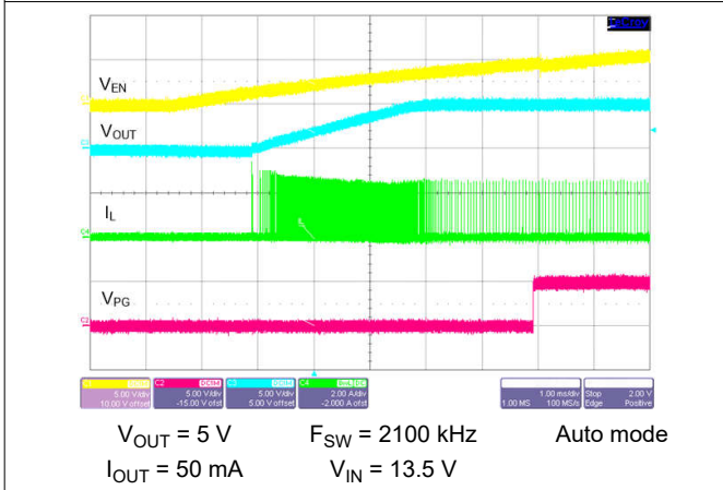
Figure 8-31. Start-up with 50-mA Load
