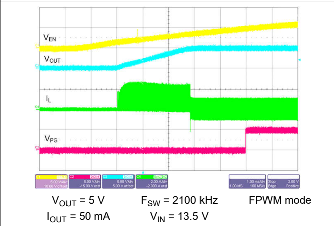
Figure 8-32. Start-up with 50-mA Load
