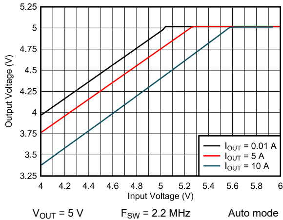
Figure 8-23. Dropout
