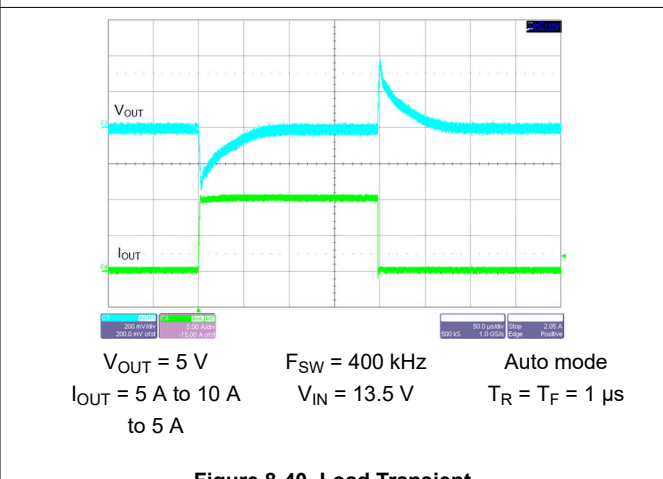
Figure 8-40. Load Transient
