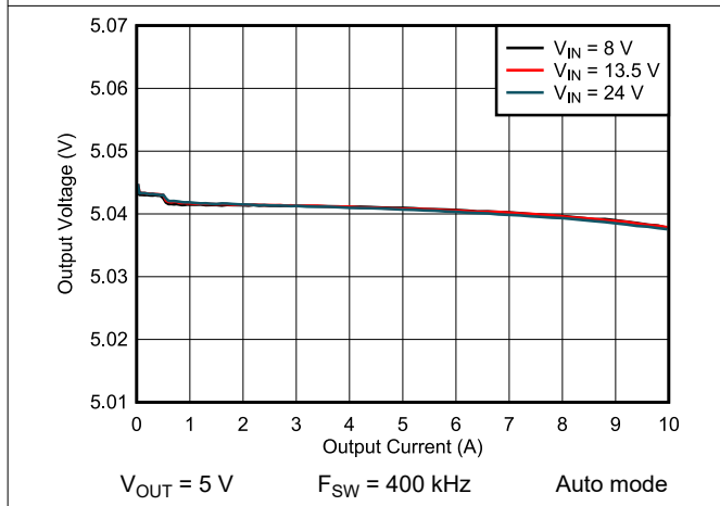
Figure 8-13. Load and Line Regulation
