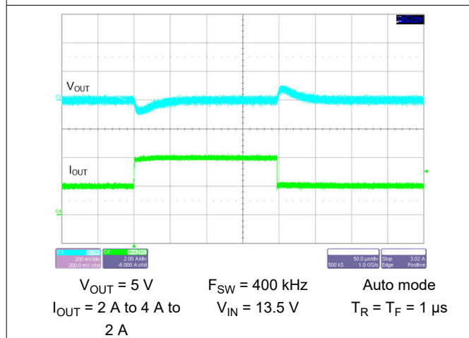
Figure 8-39. Load Transient
