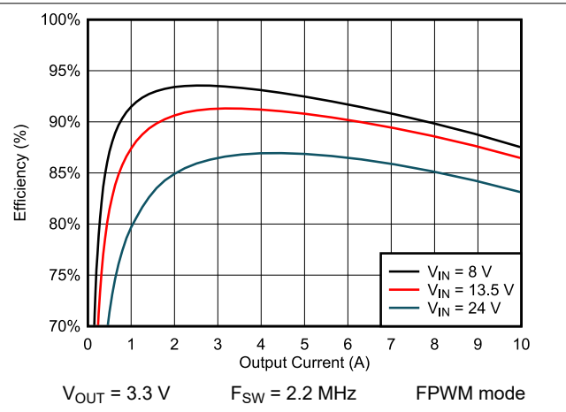
Figure 8-12. Efficiency
