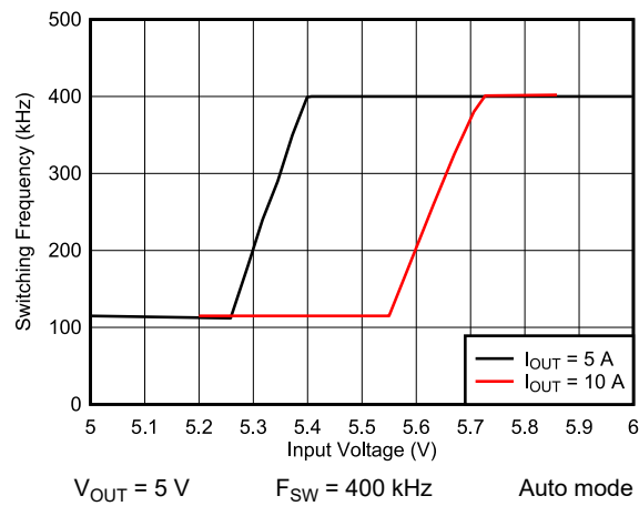
Figure 8-25. Frequency Dropout
