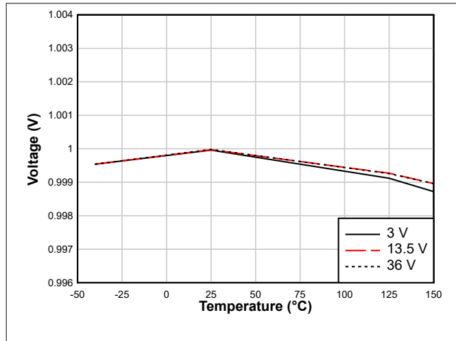
Figure 6-1. Feedback Voltage
