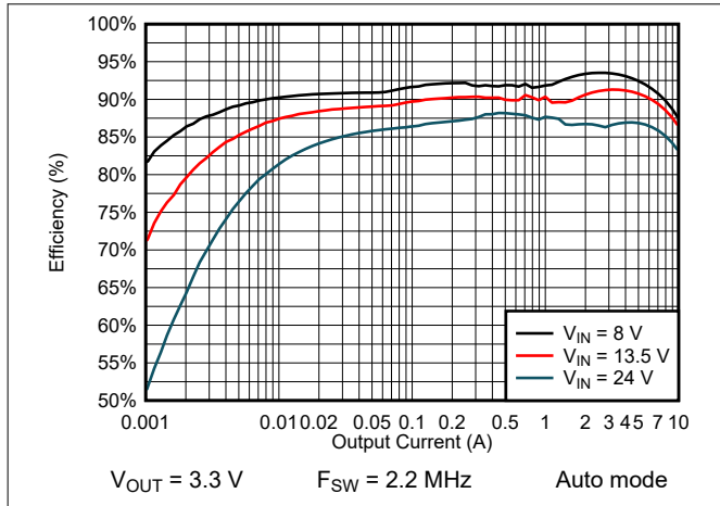
Figure 8-11. Efficiency
