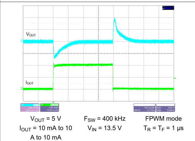
Figure 8-38. Load Transient
