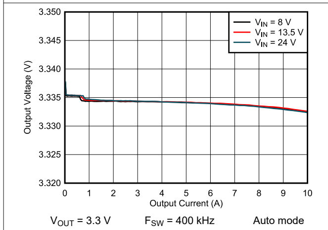
Figure 8-15. Load and Line Regulation
