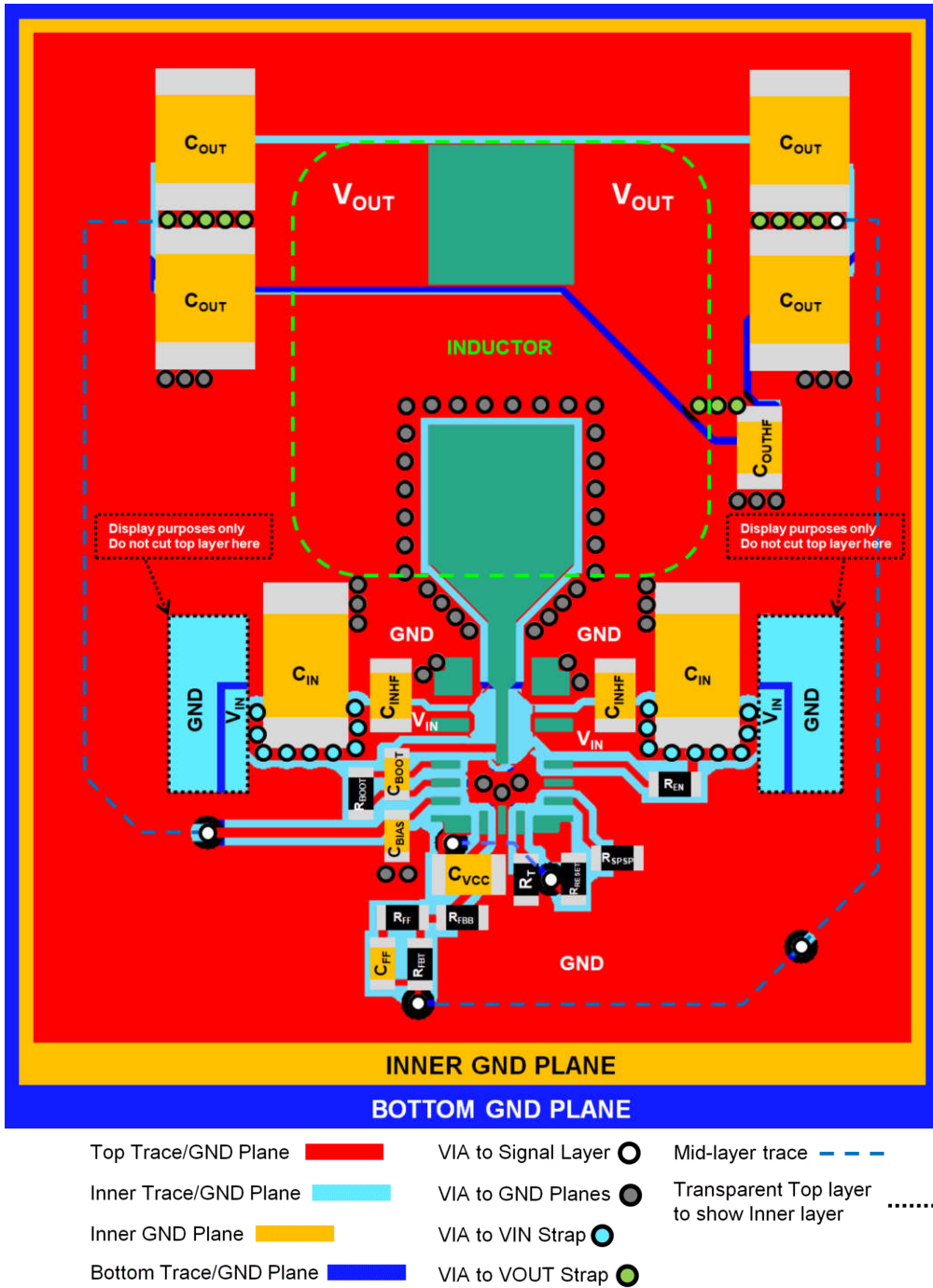
Figure 8-59. Layout Example
