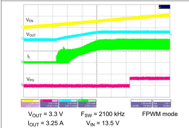
Figure 8-33. Start-up with 3.25-A Load
