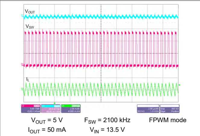
Figure 8-30. Switching Waveform and V_{OUT} Ripple
