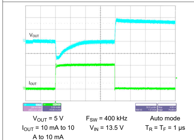
Figure 8-37. Load Transient
