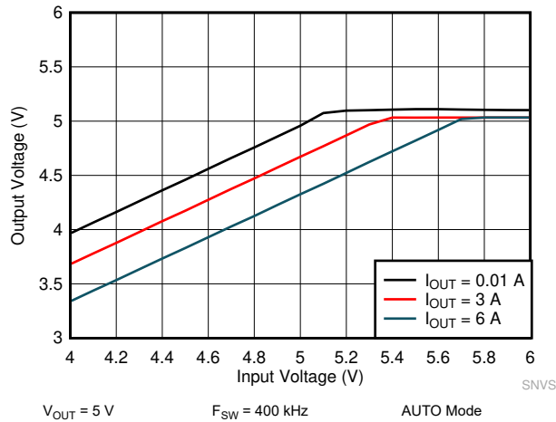
Figure 10-23. Drop Out Curve
