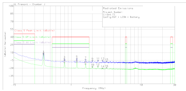
Figure 10-48. Radiated EMI Rod versus CISPR25 Limits
