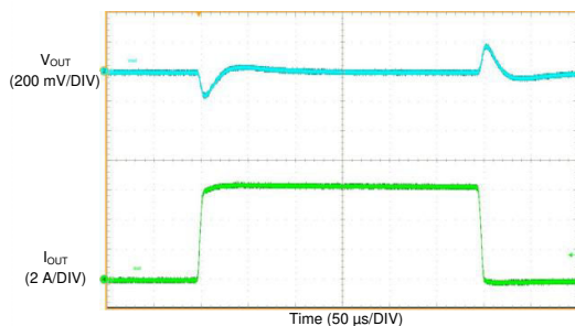
Figure 10-43. LM61460-Q1 Load Transient
