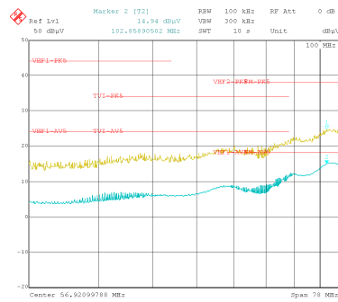
Figure 10-47. Conducted EMI versus CISPR25 Limits (Yellow: Peak Signal, Blue: Average Signal)
