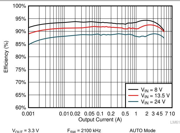
Figure 10-7. LM61460-Q1 Efficiency
