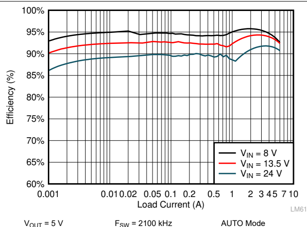
Figure 10-11. LM61460-Q1 Efficiency
