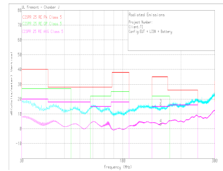
Figure 10-50. Radiated EMI Bicon Horizontal versus CISPR25 Limits
