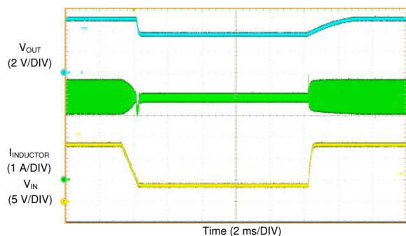
Figure 10-35. LM61460-Q1 Short Circuit Recovery
