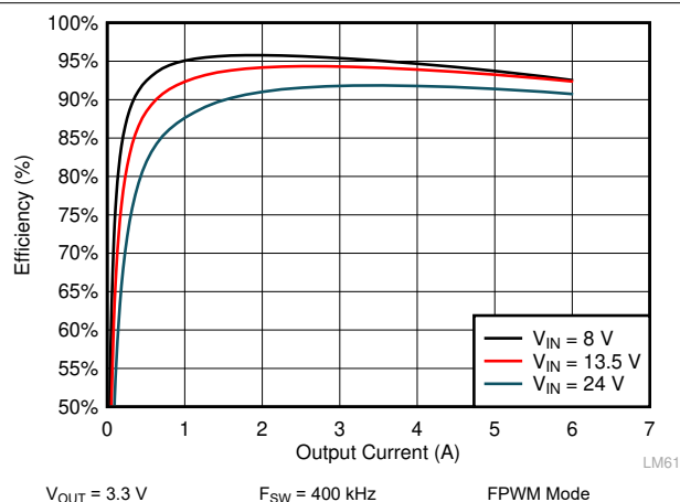
Figure 10-6. LM61460-Q1 Efficiency
