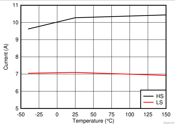
Figure 8-4. LM61460-Q1 High-side and Low-side Current Limits
