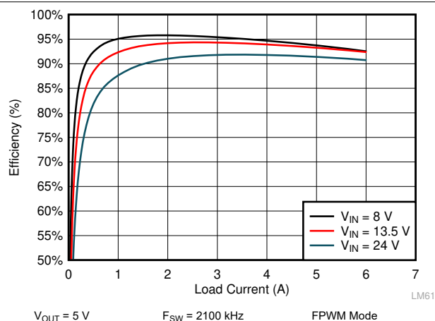
Figure 10-12. LM61460-Q1 Efficiency
