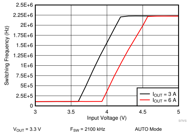
Figure 10-26. LM61460-Q1 Frequency Dropout Curve
