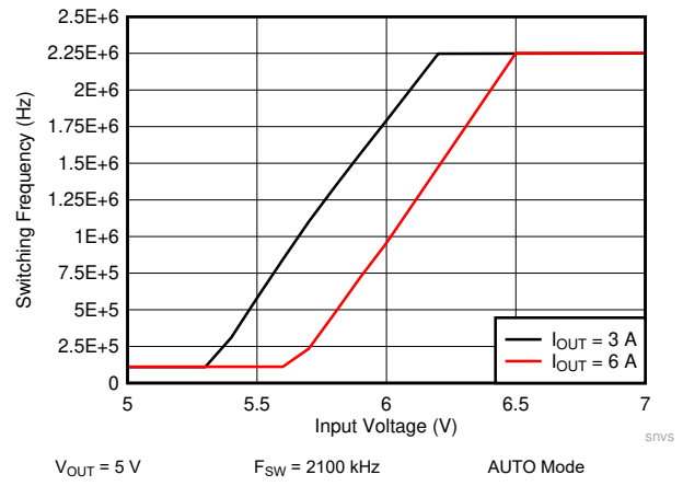
Figure 10-28. LM61460-Q1 Frequency Dropout Curve
