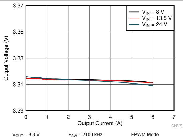
Figure 10-16. LM61460-Q1 Load and Line Regulation
