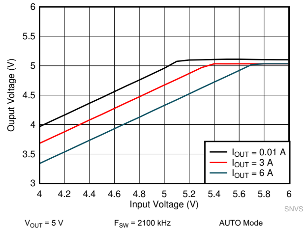
Figure 10-24. LM61460-Q1 Drop Out Curve
