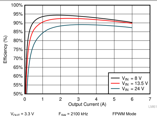
Figure 10-8. LM61460-Q1 Efficiency
