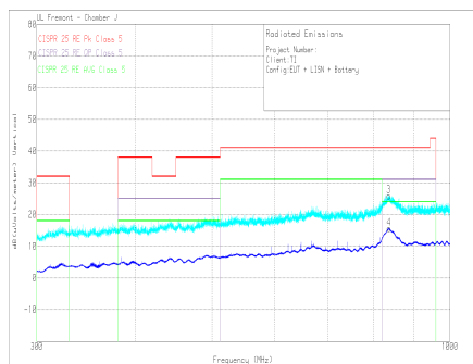
Figure 10-49. Radiated EMI Bicon Vertical versus CISPR25 Limits
