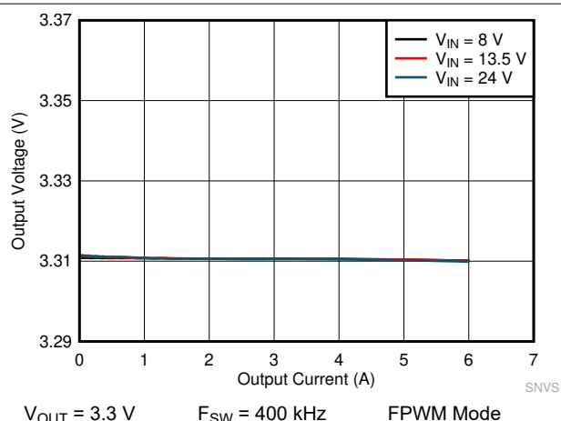
Figure 10-14. LM61460-Q1 Load and Line Regulation
