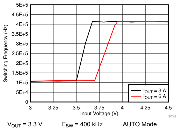
Figure 10-25. LM61460-Q1 Frequency Dropout Curve
