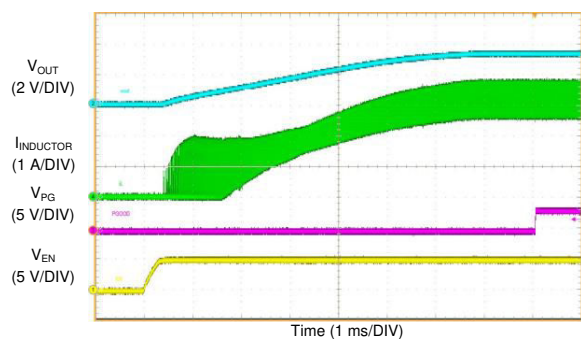
Figure 10-31. LM61460-Q1 Start-up with 50-mA Load
