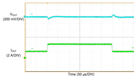
Figure 10-41. LM61460-Q1 Load Transient
