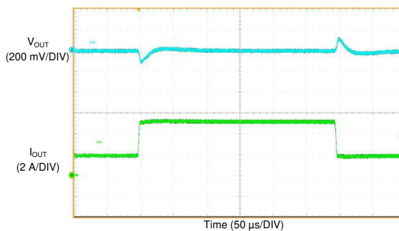
Figure 10-38. LM61460-Q1 Load Transient
