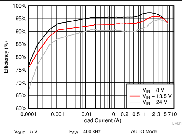
Figure 10-9. LM61460-Q1 Efficiency
