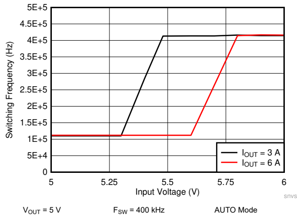
Figure 10-27. LM61460-Q1 Frequency Dropout Curve
