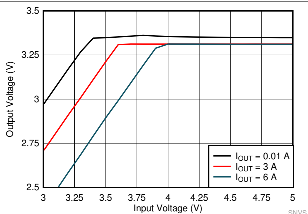
Figure 10-20. LM61460-Q1 Load and Line Regulation
