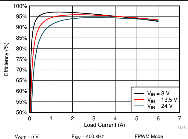
Figure 10-10. LM61460-Q1 Efficiency
