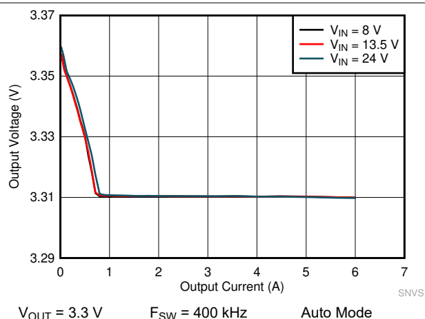
Figure 10-13. LM61460-Q1 Load and Line Regulation
