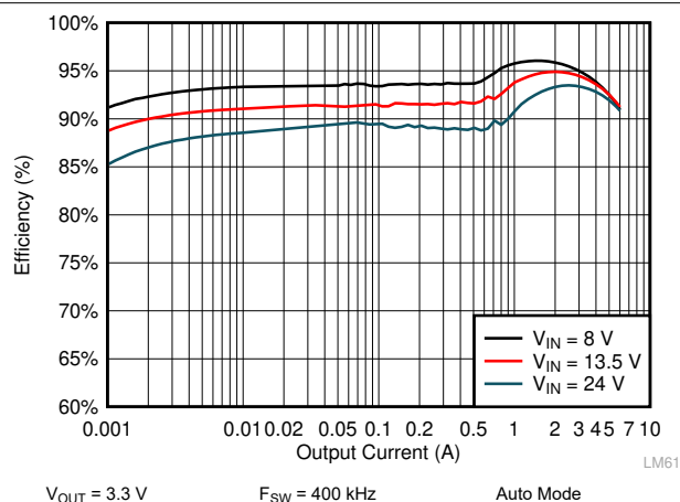
Figure 10-5. LM61460-Q1 Efficiency
