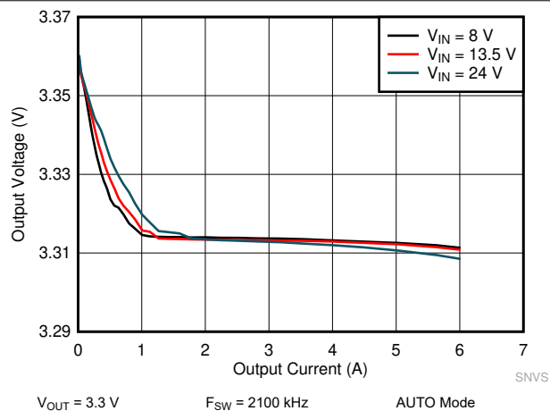
Figure 10-15. LM61460-Q1 Load and Line Regulation
