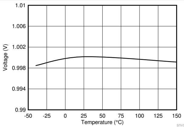
Figure 8-3. Feedback Voltage
