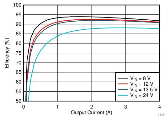
Figure 10-6. LM61440-Q1 Efficiency
