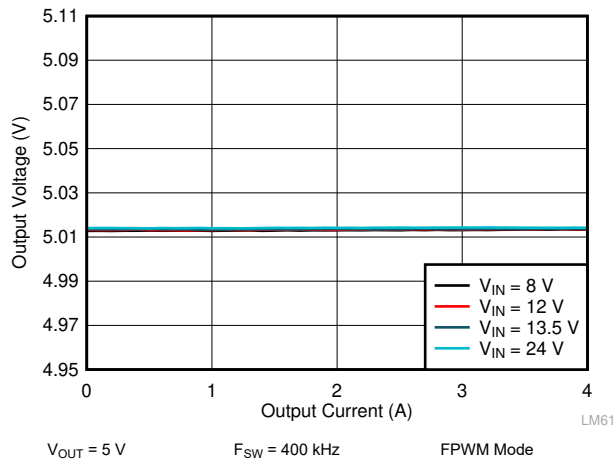
Figure 9-13. LM61440 Load and Line Regulation
