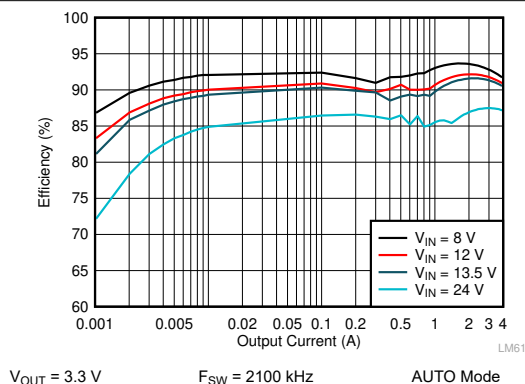
Figure 9-5. LM61440 Efficiency
