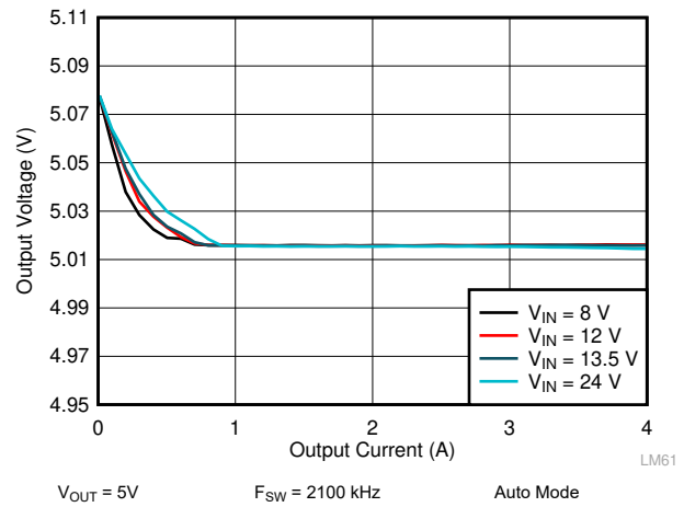
Figure 9-14. LM61440 Load and Line Regulation
