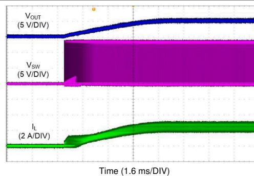
Figure 9-26. LM61440 Start-up with 3.25-A
