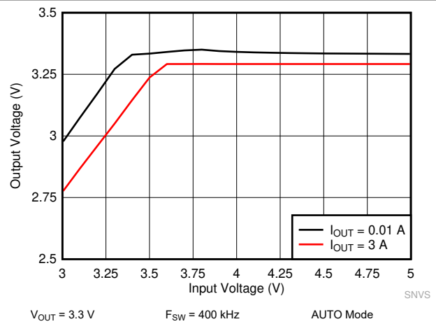
Figure 9-16. LM61440 Dropout Curve
