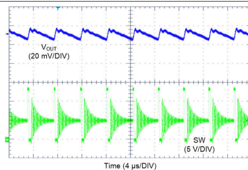
Figure 9-24. LM61440 Switching Waveform and V_{OUT} Ripple
