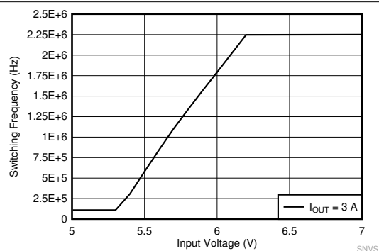
Figure 9-23. LM61440 Frequency Dropout Curve
