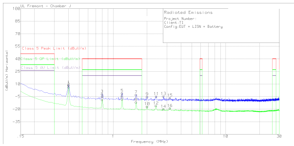
Figure 9-35. Radiated EMI Rod versus CISPR25 Limits
