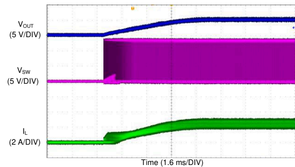
Figure 8-14. Short Circuit Recovery
