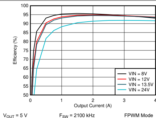
Figure 9-7. LM61440-Q1 Efficiency
