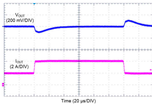
Figure 9-32. LM61440 Load Transient
