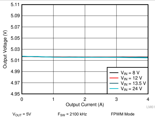
Figure 9-15. LM61440 Load and Line Regulation
