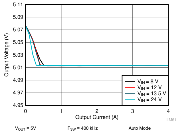
Figure 9-12. LM61440 Load and Line Regulation
