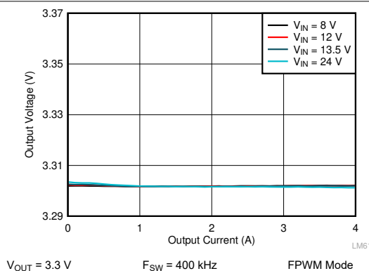
Figure 9-9. LM61440 Load and Line Regulation
