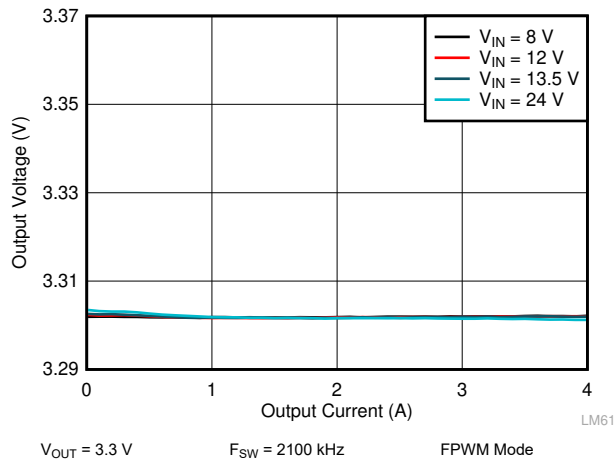
Figure 9-11. LM61440 Load and Line Regulation
