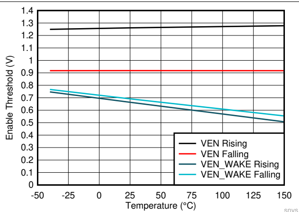
Figure 7-6. Enable Thresholds
