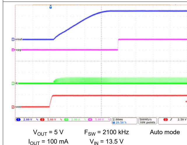
Figure 9-32. LM61430-Q1 Start-up with 100-mA Load
