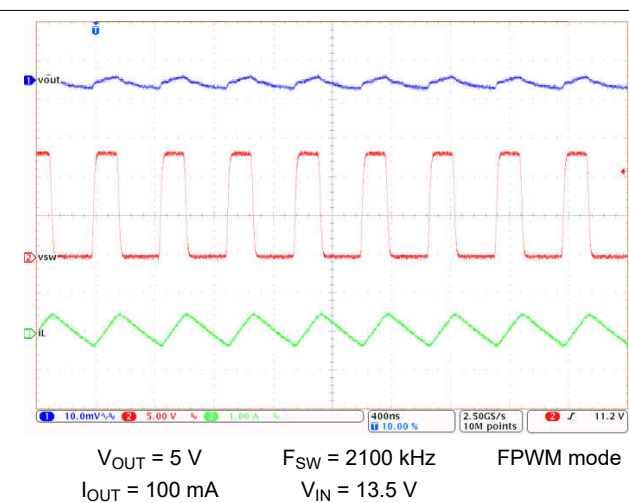
Figure 9-29. LM61430-Q1 Switching Waveform and V_{OUT} Ripple
