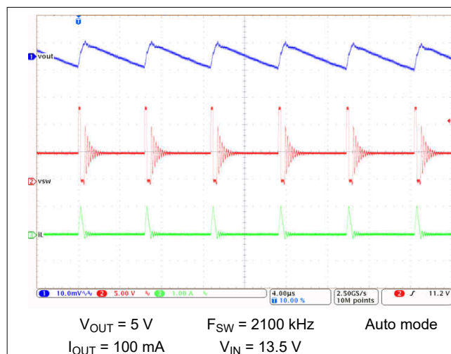
Figure 9-28. LM61430-Q1 Switching Waveform and V_{OUT} Ripple
