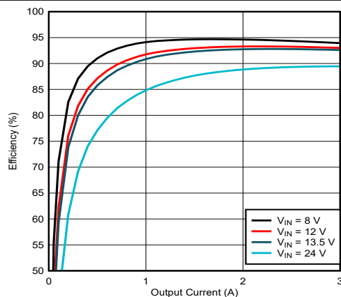
Figure 9-11. LM61430-Q1 Efficiency
