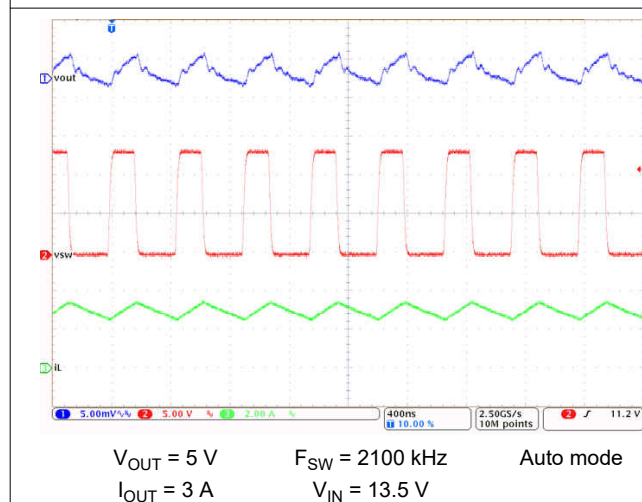
Figure 9-30. LM61430-Q1 Switching Waveform and V_{OUT} ripple
