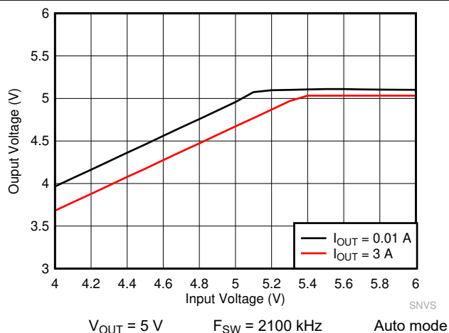
Figure 9-23. LM61430-Q1 Dropout Curve
