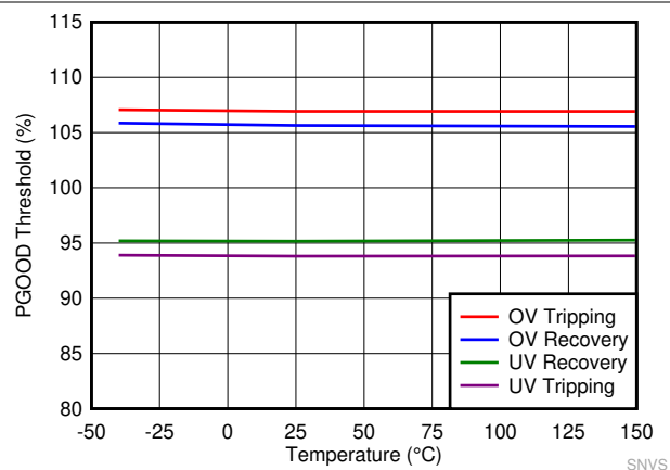
Figure 7-7. PGOOD Thresholds
