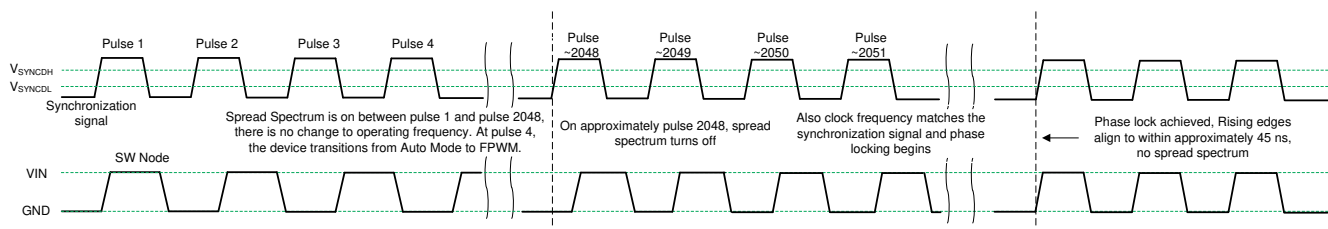
Figure 8-4. Synchronization Process
