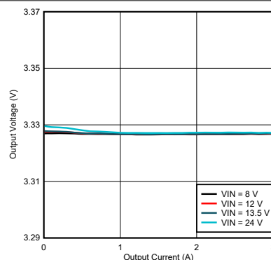
Figure 9-15. LM61430-Q1 Load and Line Regulation
