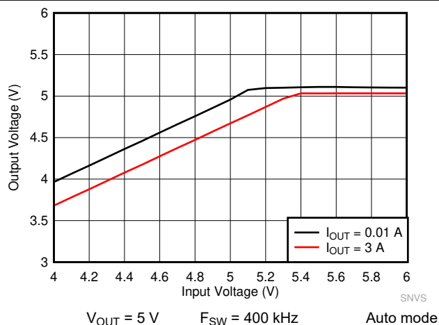
Figure 9-22. LM61430-Q1 Dropout Curve
