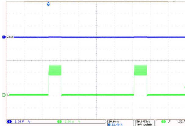
Figure 8-12. Inductor Current Bursts During Hiccup
