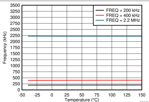
Figure 7-4. Switching Frequency Set by RT Resistor
