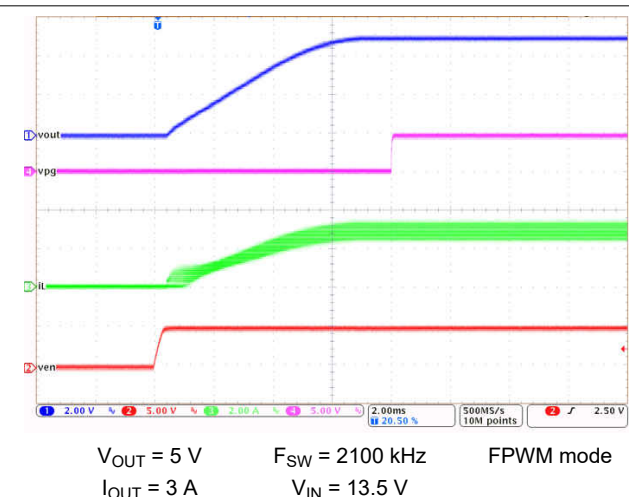
Figure 9-33. LM61430-Q1 Start-up with 3 A
