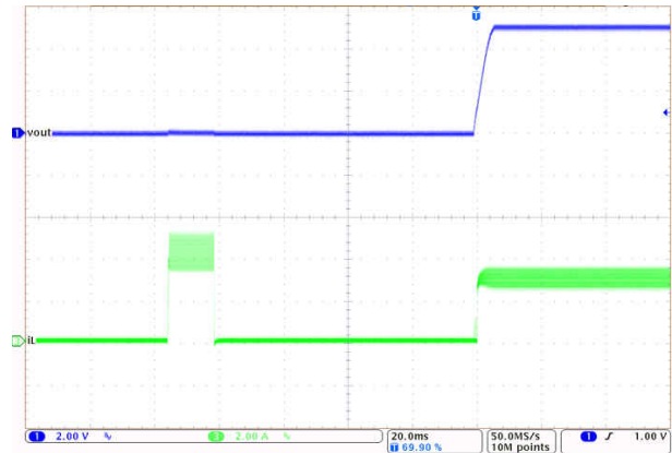
Figure 8-13. Short-Circuit Recovery
