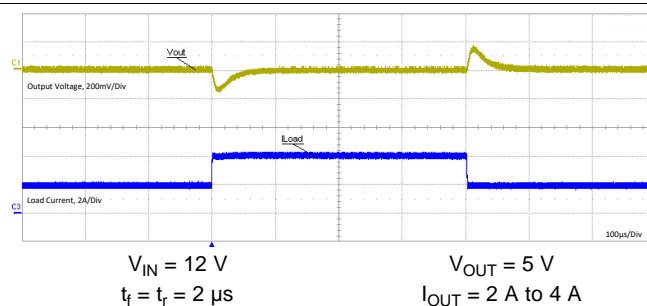
Figure 22. Load Transient
