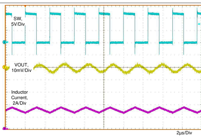
Figure 14. LM60430-Q1 Typical PWM Switching Waveforms V_{IN} = 12\text{ V} , V_{OUT} = 5\text{ V} , I_{OUT} = 3\text{ A} , f_s = 400\text{ kHz}
