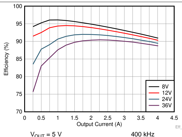
Figure 18. High-Load Efficiency
