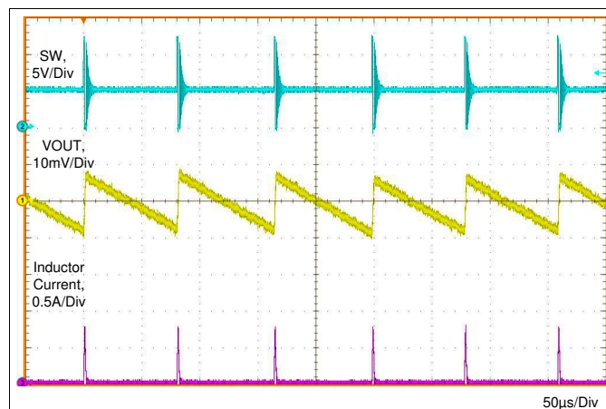
Figure 13. LM60430-Q1 Typical PFM Switching Waveforms V_{IN} = 12\text{ V} , V_{OUT} = 5\text{ V} , I_{OUT} = 10\text{ mA}
