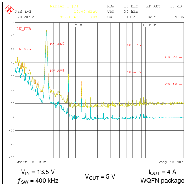
Figure 24. Low Frequency Conducted EMI
