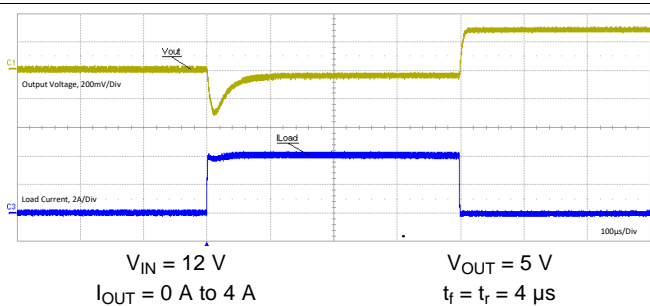
Figure 21. Load Transient
