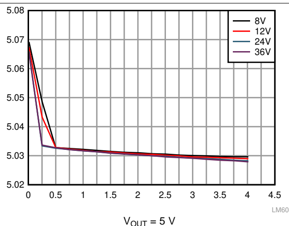
Figure 19. Line and Load Regulation
