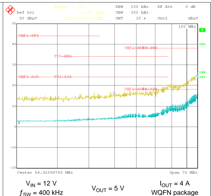
Figure 25. High Frequency Conducted EMI
