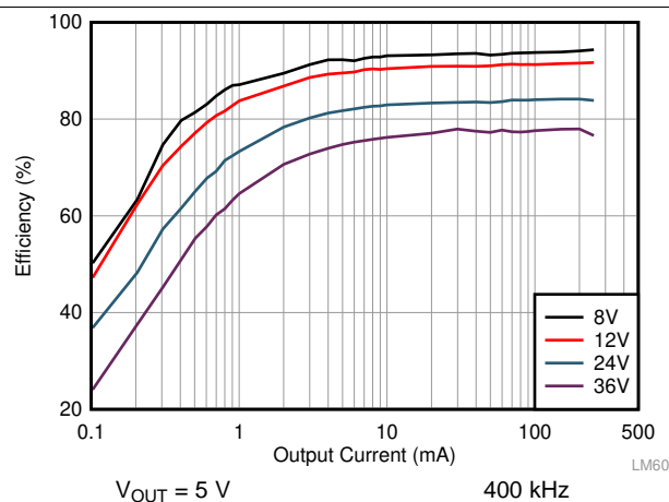
Figure 17. Low-Load Efficiency
