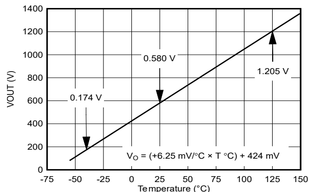
Full-Range Centigrade Temperature Sensor ( -40^{\circ}\text{C} to +125^{\circ}\text{C} )
