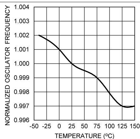
Figure 2. Oscillator Frequency vs Temperature F_{\text{OSC}} = 200\text{ kHz}
