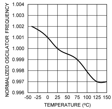
Figure 5-2. Oscillator Frequency vs Temperature F_{OSC} = 200kHz
