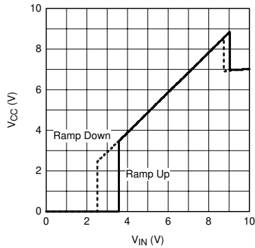
Figure 5-5. V_{CC} vs V_{IN} R_L = 7k\Omega
