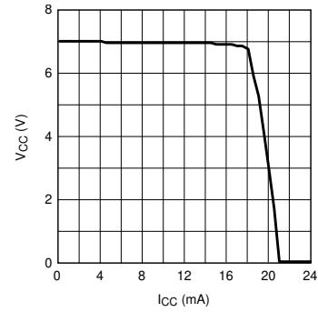
Figure 5-4. V_{CC} vs I_{CC} V_{IN} = 12V
