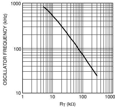
Figure 5-1. Oscillator Frequency vs R_T
