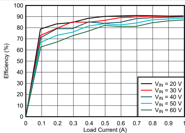
Figure 8-2. Efficiency
