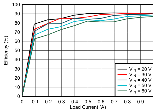
Typical Efficiency, V_{OUT} = 16.4\text{ V}
