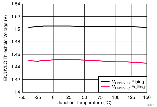
Figure 7-10. EN/UVLO Threshold Voltages versus Temperature
