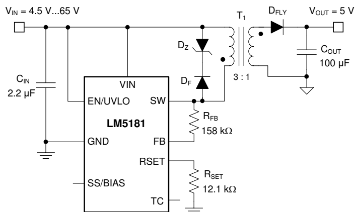
Typical Application
