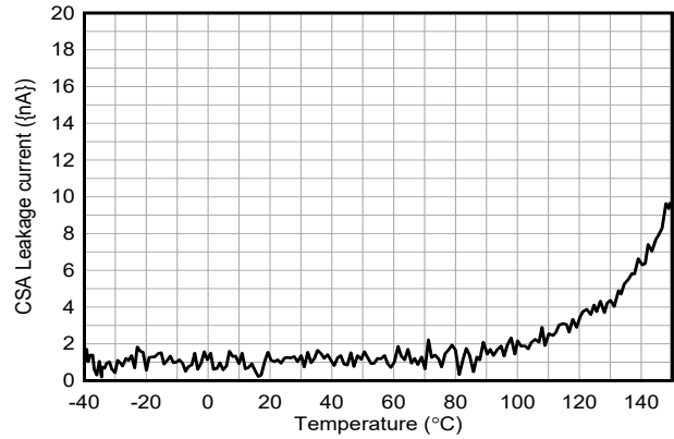
Figure 5-26. CSA Input Current versus Temperature
