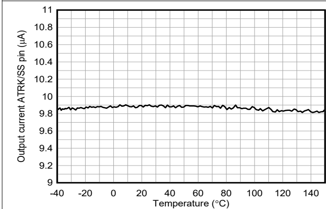
Figure 5-15. Soft-Start current versus Temperature
