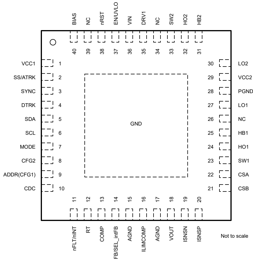
Figure 4-1. LM51772-Q1RHA Package, 40-Pin QFN (Top View)
