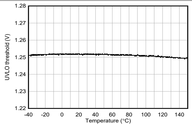
Figure 5-16. EN/UVLO Threshold versus Temperature
