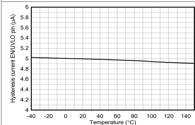
Figure 5-17. Hysteresis Current on EN/UVLO versus Temperature
