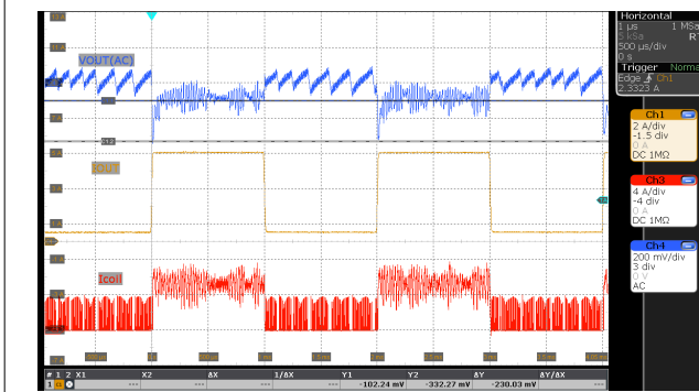
Figure 9-22. Load transient ( V_{(VIN)} = 24V , V_{(VOUT)} = 24V I_O = 0.5A \leftrightarrow 5A , MODE = GND )
