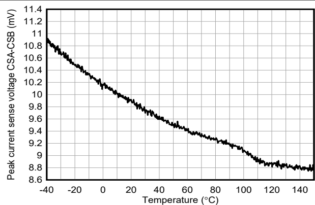
Figure 5-30. Average Current Limit Threshold Voltage Versus Temperature ILIM_THRESHOLD = 0x14
