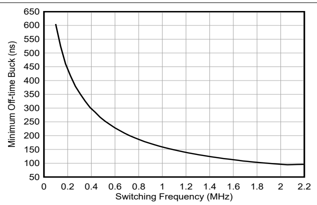
Figure 5-18. Buck Minimum Off-time versus Switching Frequency
