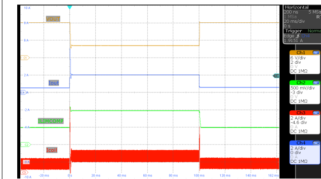
Figure 9-24. Average Output Current Limit ( V_{(VIN)} = 12V , V_{(VOUT)} = 12V I_O = 0.5A \leftrightarrow 5A , MODE = VCC2, ILIM_THRESHOLD = 0x28 (2A) )
