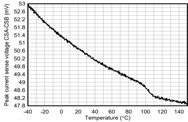
Figure 5-28. Average Current Limit Threshold Voltage Versus Temperature ILIM_THRESHOLD = 0x64
