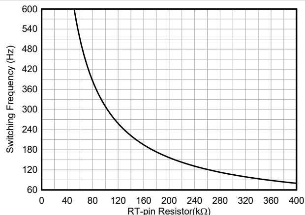
Figure 5-1. Switching Frequency Versus R_T Resistance
