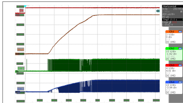
Figure 8-2. Start-up waveform standby to active operation (MODE = V VCC , V O = 12 V, I O = 0 A, V VIN = 12 V)
