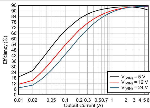
Figure 8-11. Efficiency Versus I_o (MODE = VCC V_o = 12 V)
