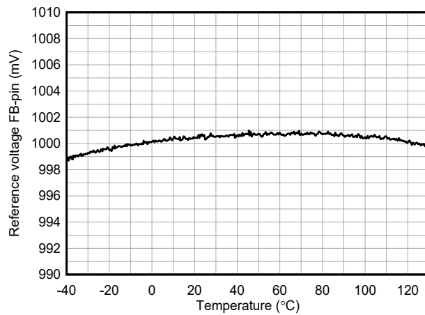
Figure 5-7. FB Pin Reference Voltage versus Temperature
