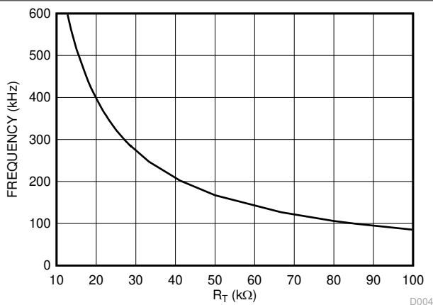
Figure 6-3. Oscillator Frequency
