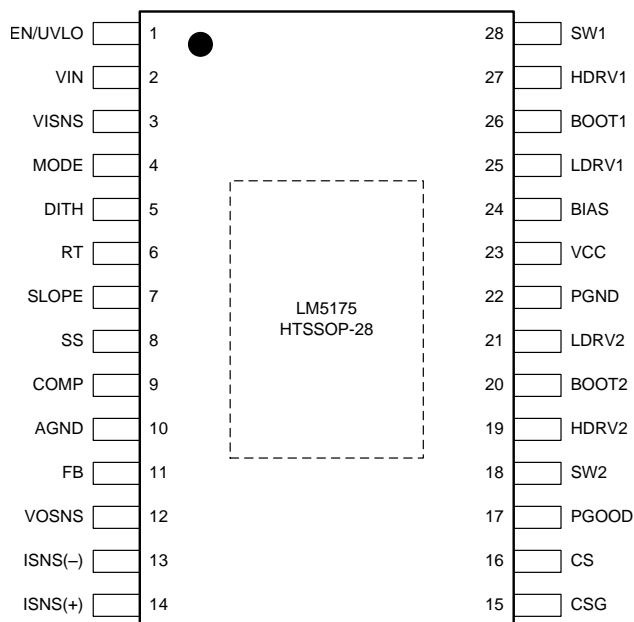
HTSSOP-28 PWP Package Top View
