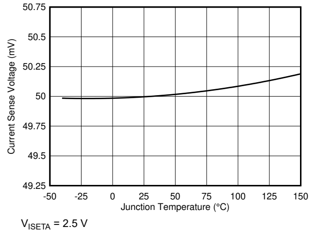
Figure 7-8. Regulated V_{CS} Voltage vs Temperature
