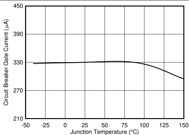
Figure 7-18. Circuit Breaker Gate Current vs Temperature
