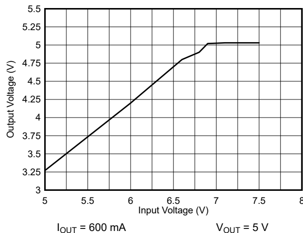
Figure 8-31. Drop-Out Response
