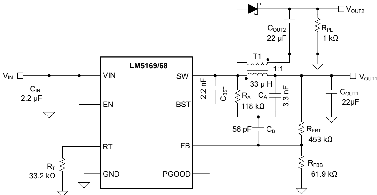
Figure 8-1. Example Fly-Buck™ Converter Application Circuit
