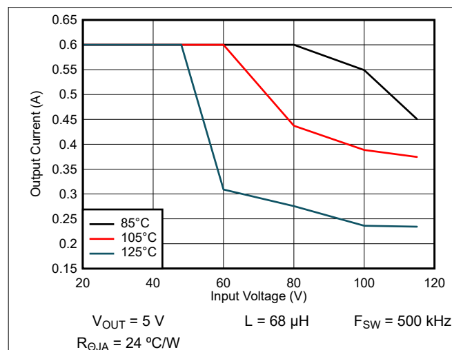
Figure 8-35. Maximum Output Current: V_{OUT} = 5\text{ V}
