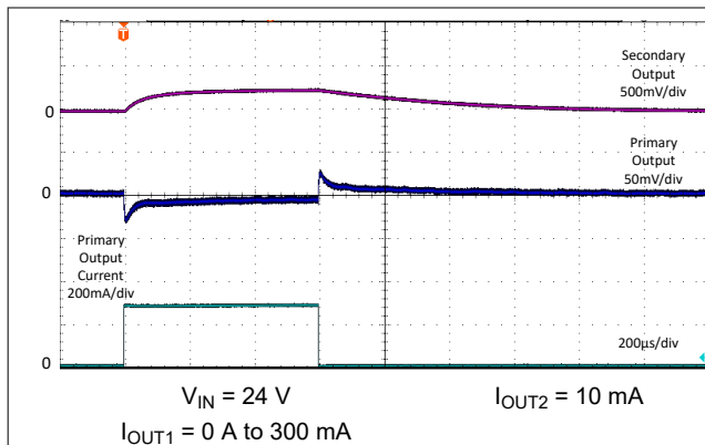
Figure 8-8. Load Transient on Primary Output
