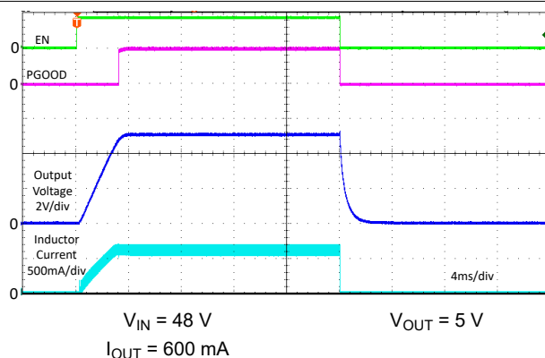
Figure 8-29. Typical Start-up Waveforms
