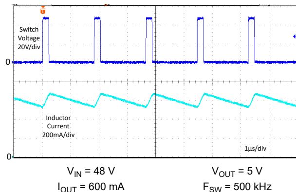
Figure 8-27. Typical Switching Waveforms
