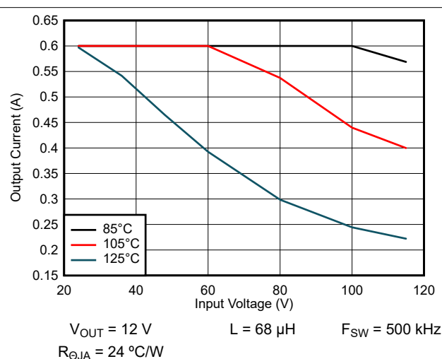
Figure 8-36. Maximum Output Current: V_{OUT} = 12\text{ V}
