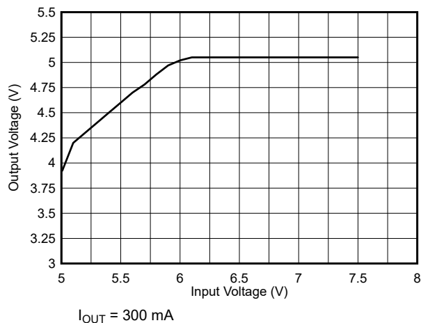
Figure 8-32. Drop-Out Response
