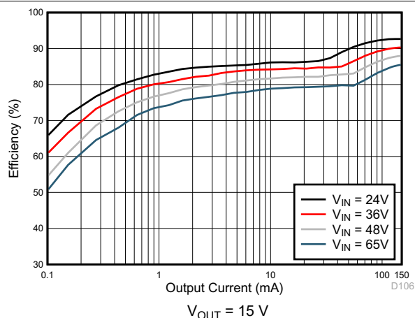
Figure 8-30. Efficiency
