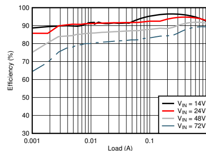
Typical Application Efficiency, V OUT = 12V
