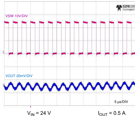
Figure 7-15. Full-Load Switching
