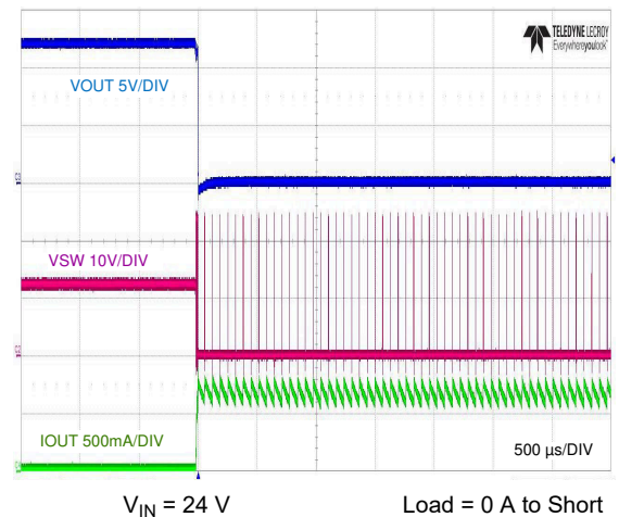
Figure 7-11. Short Circuit Applied
