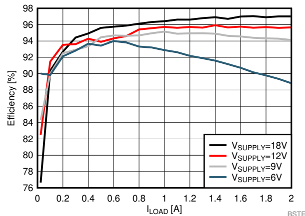
Figure 10-2. Efficiency
