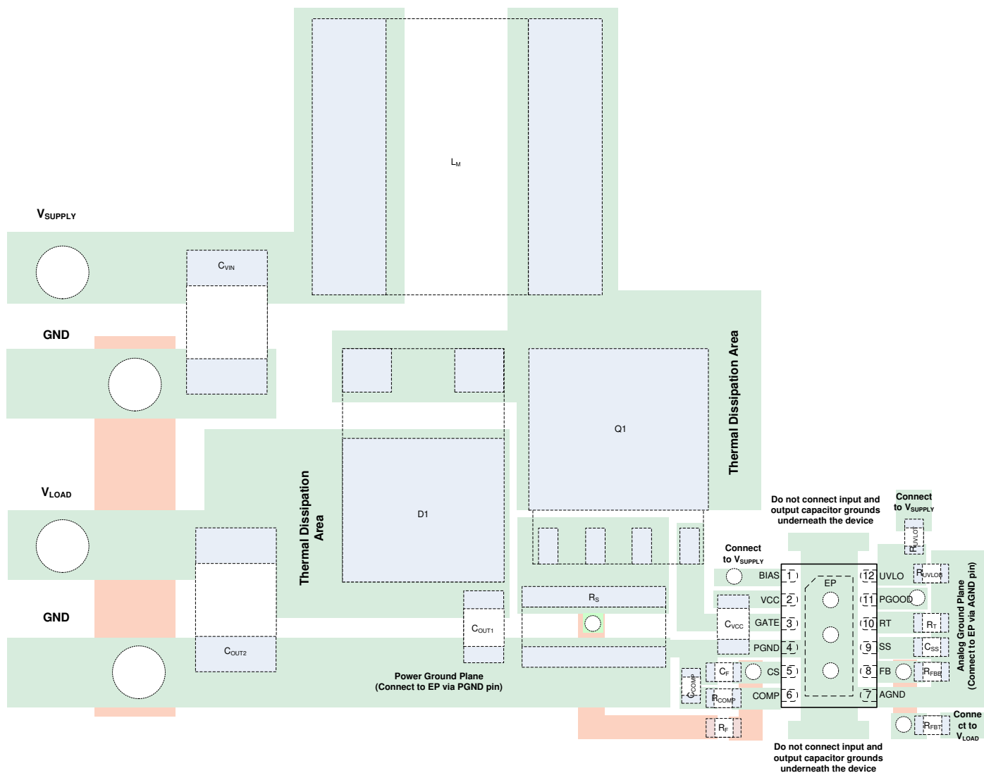
Figure 10-16. PCB Layout Example 2
