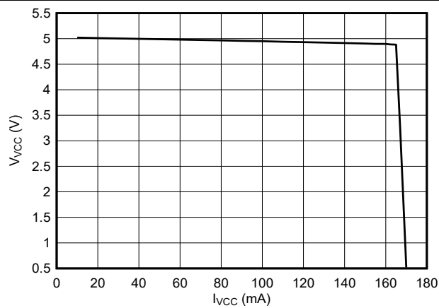
Figure 8-9. V VCC vs I VCC
