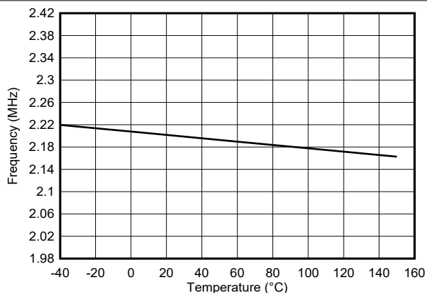
Figure 8-2. Frequency vs Temperature (RT = 9.09 kΩ, 2.2 MHz)
