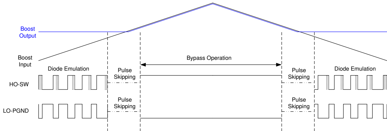
Figure 9-19. PWM to Bypass Transition in DCM Operation
