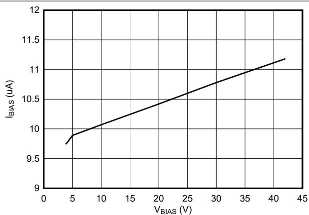
Figure 8-6. VBIAS vs IBIAS (Bypass Mode, Charge Pump Off)
