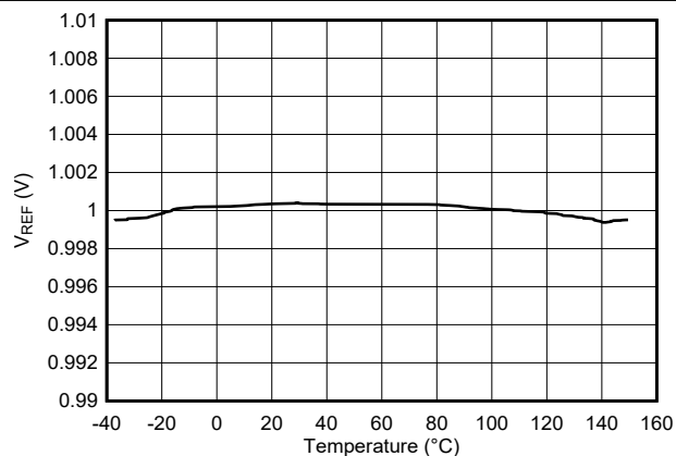
Figure 8-16. V_{REF} vs Temperature
