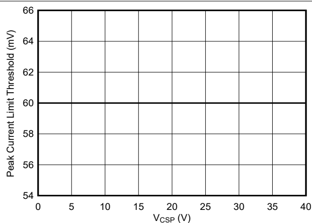
Figure 8-11. Peak Current Limit Threshold vs V CSP
