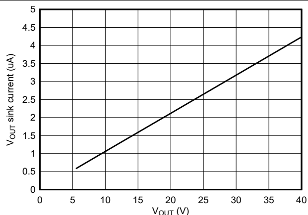
Figure 8-14. V_{OUT} Sink Current vs V_{OUT} (Deep Sleep)
