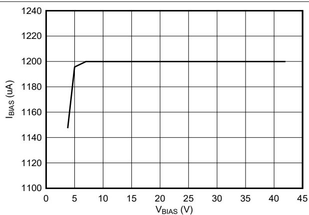
Figure 8-4. VBIAS vs IBIAS (Active Mode)
