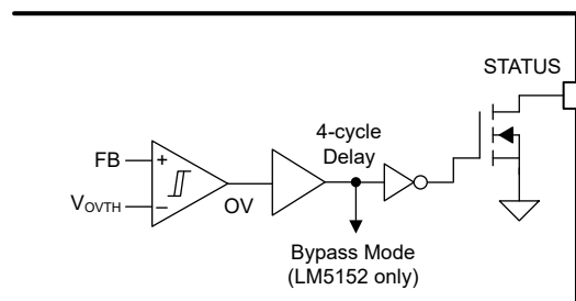
Figure 9-7. STATUS Indicator
