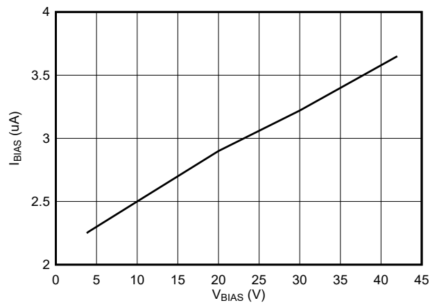
Figure 8-7. V BIAS vs I BIAS (Shutdown Mode)
