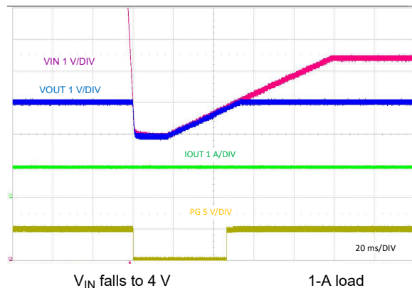
Figure 8-34. Cold-Crank Response to V_{IN} = 4 V
