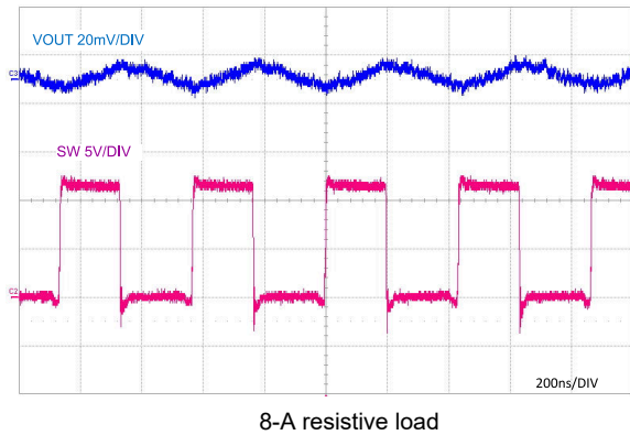
Figure 8-7. Full Load Switching
