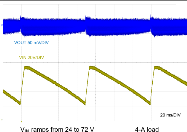
Figure 8-23. Line Transient Response to V_{IN} = 72\text{ V}
