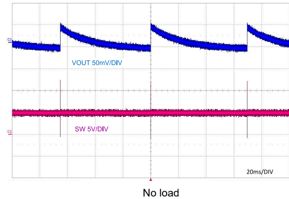
Figure 8-8. PFM Switching
