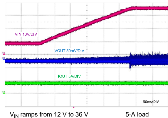
Figure 8-9. Line Transient
