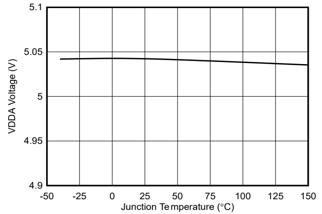
Figure 6-14. VDDA Regulation Voltage vs Temperature
