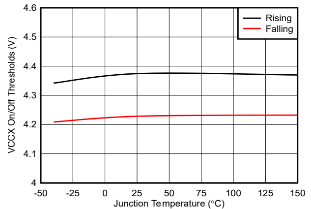
Figure 6-16. VCCX On, Off Thresholds vs Temperature
