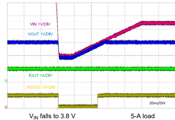
Figure 8-10. Cold-Crank Response to V_{IN} = 3.8 V
