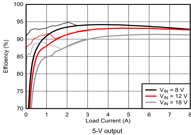
Figure 8-5. Efficiency vs I_{OUT}
