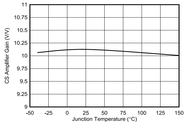
Figure 6-18. Current Sense (CS) Amplifier Gain vs Temperature
