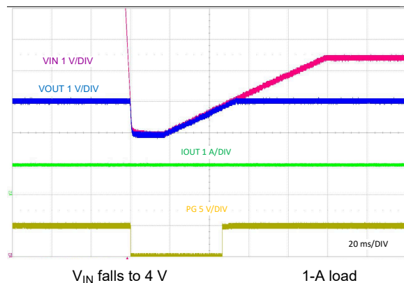
Figure 9-34. Line Transient Response to V_{IN} = 4 V
