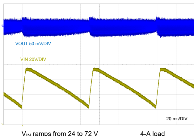
Figure 9-23. Line Transient Response to V_{IN} = 72\text{ V}
