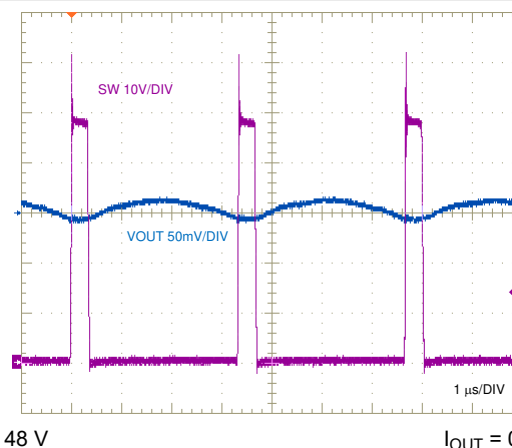
Figure 9-15. SW Node and Output Ripple Voltages
