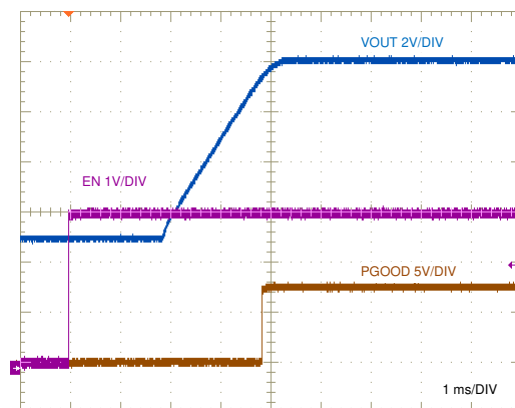
Figure 9-28. Pre-Biased Start-Up
