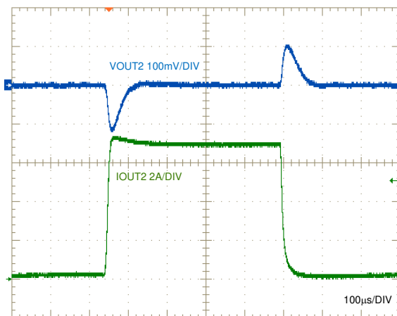
V_{IN} = 12 V PWM Figure 10-15. Load Transient, 5-V Output, 0 A to 7 A
