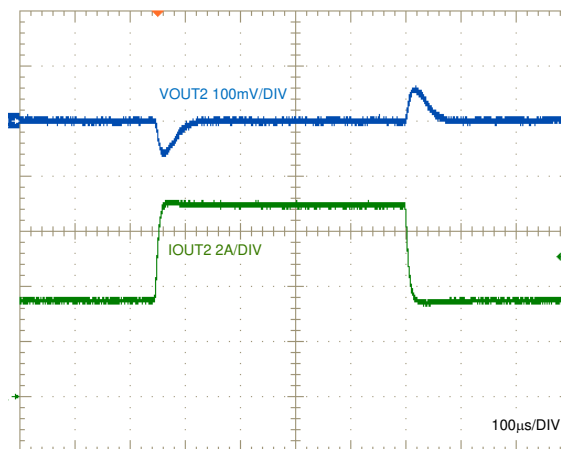
V_{IN} = 12 V PWM Figure 10-16. Load Transient, 5-V Output, 3.5 A to 7 A
