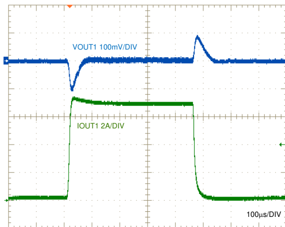
V_{IN} = 12 V PWM Figure 10-13. Load Transient, 3.3-V Output, 0 A to 7 A
