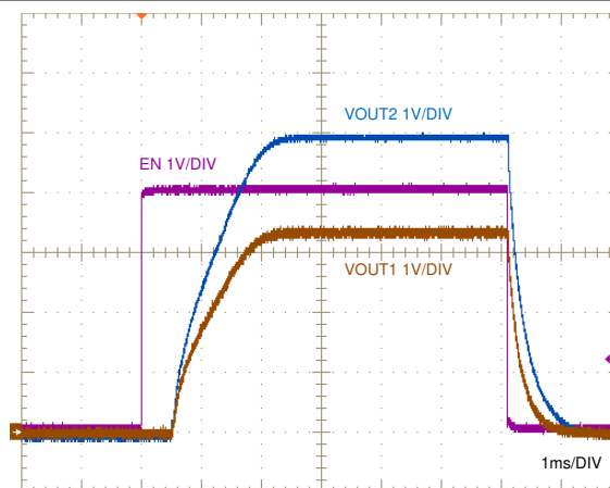
V_{IN} = 12 V 7-A resistive loads Figure 10-12. ENABLE ON and OFF Characteristic
