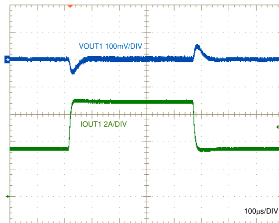
V_{IN} = 12 V PWM Figure 10-14. Load Transient, 3.3-V Output, 3.5 A to 7 A
