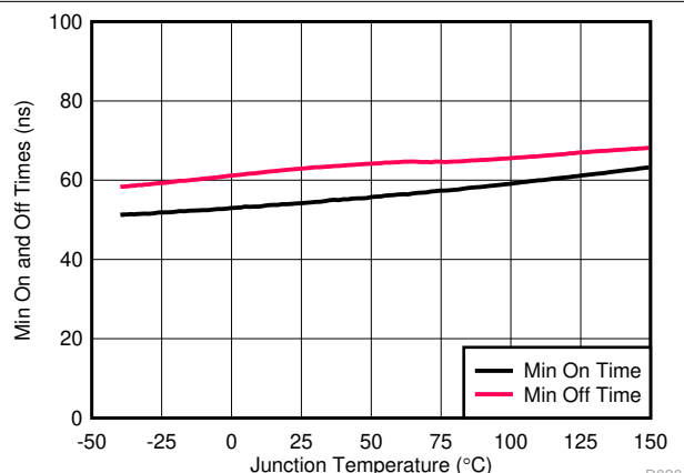
Figure 7-24. Minimum On Time and Off Time (HO1) versus Temperature
