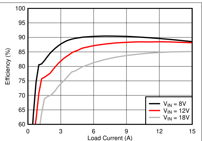
Figure 9-23. Efficiency versus I OUT , 3.3-V Output
