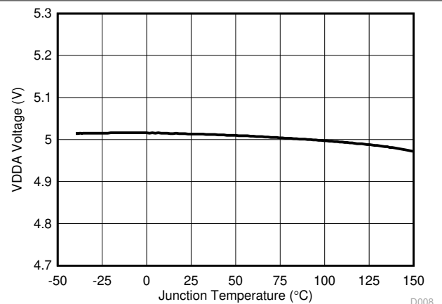
Figure 7-18. VDDA Regulation Voltage versus Temperature
