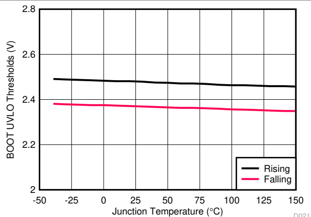
Figure 7-25. BOOT (HB1) UVLO Thresholds versus Temperature
