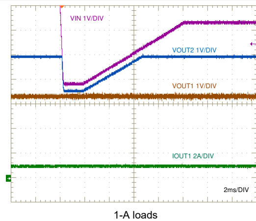
Figure 9-10. Cold-Crank Response to V_{IN} = 3.8\text{ V}
