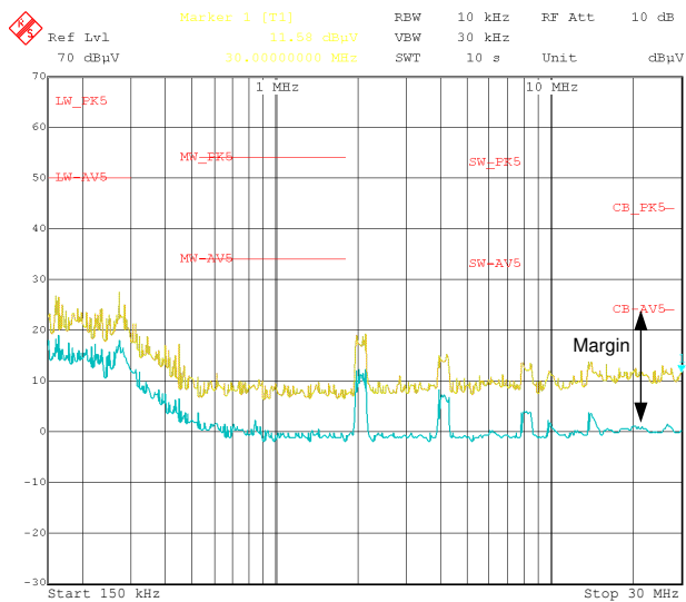
V_{IN} = 13.5\text{ V} V_{OUT} = 5\text{ V} 7-A resistive load Figure 9-19. CISPR 25 Class 5 Conducted EMI, 150 kHz to 30 MHz
