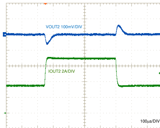
Figure 9-14. Load Transient, 3.3-V Output, 3.5 A to 7 A
