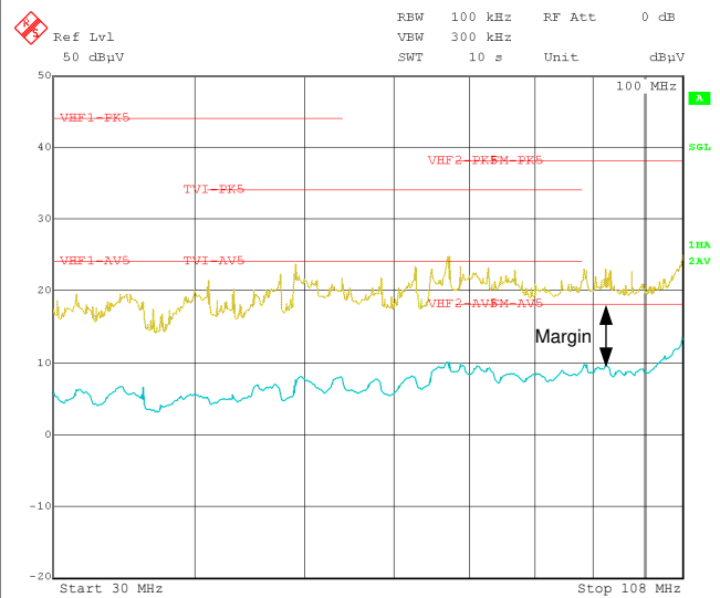
V_{IN} = 13.5\text{ V} V_{OUT} = 5\text{ V} 7-A resistive load Figure 9-20. CISPR 25 Class 5 Conducted EMI, 30 MHz to 108 MHz
