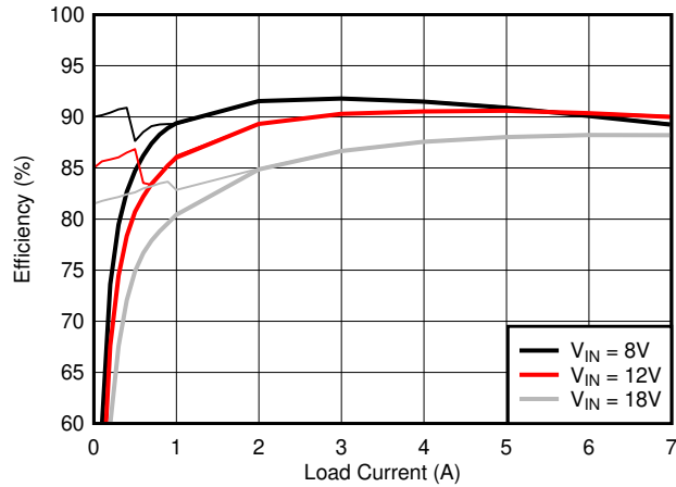
Figure 9-5. Efficiency versus I_{OUT}
