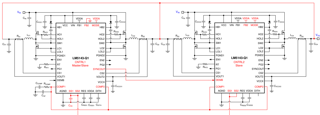
Figure 8-10. Multiphase Regulator Schematic Configured for Single-Output Interleaved Operation
