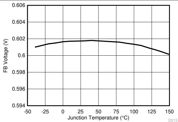
Figure 7-12. Feedback Voltage versus Temperature
