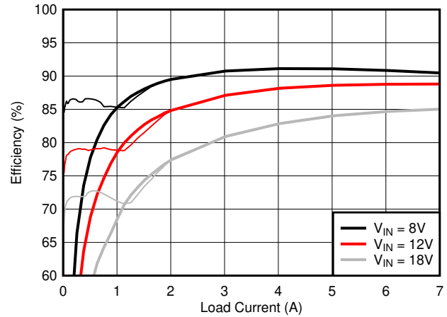
Figure 9-6. Efficiency versus I_{OUT}
