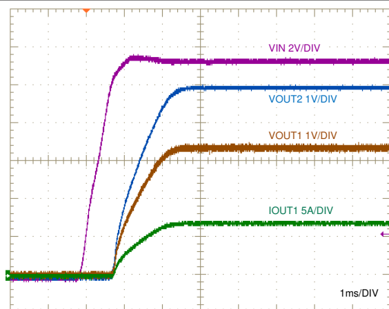
Figure 9-11. Start-Up Characteristic
