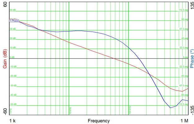
V_{IN} = 12\text{ V} 7-A resistive load Figure 9-17. Bode Plot, 3.3-V Output
