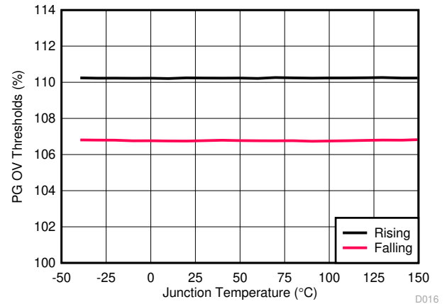
Figure 7-14. PG OV Thresholds versus Temperature
