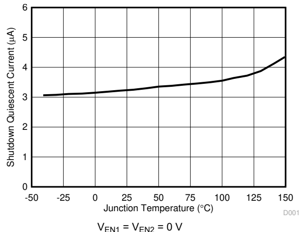
Figure 7-6. Shutdown Current versus Temperature
