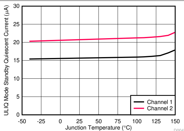
Figure 7-9. ULIQ Mode Standby Current versus Temperature
