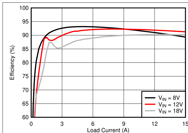
Figure 9-22. Efficiency versus I OUT , 5-V Output
