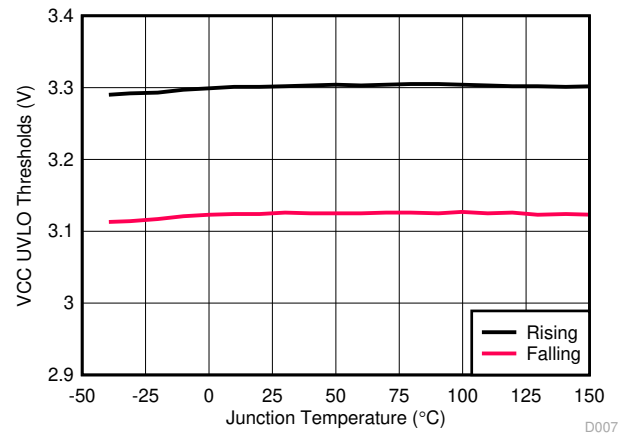
Figure 7-16. VCC UVLO Thresholds versus Temperature
