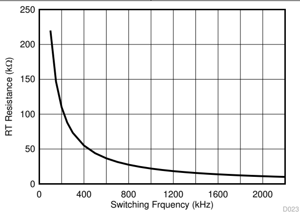
Figure 7-27. RT Resistance versus Switching Frequency
