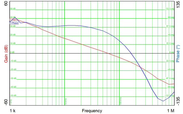
V_{IN} = 12\text{ V} 7-A resistive load Figure 9-18. Bode Plot, 5-V Output
