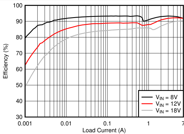
Figure 9-7. Efficiency versus I_{OUT} , Log Scale
