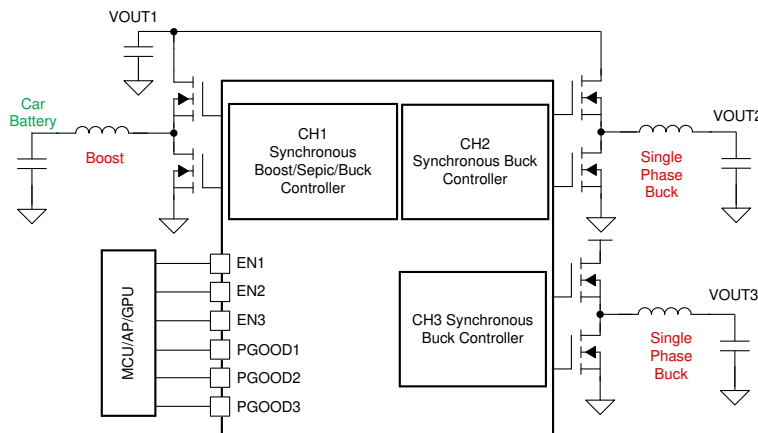
Typical Application (Pre-boost + Two bucks)
