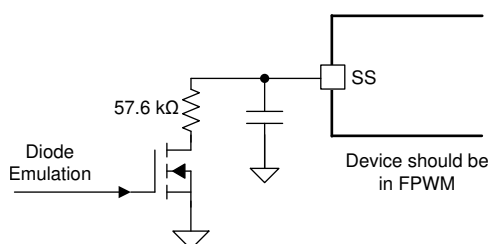
Figure 9-4. Dynamic Transition Between FPWM and DE
