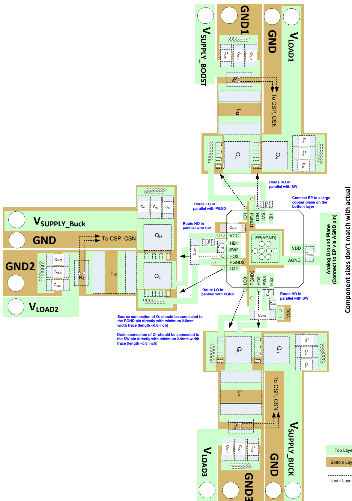
Figure 11-1. PCB Layout Example
