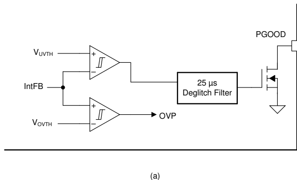
Figure 8-5. Power Good Monitor (a) Boost configuration
