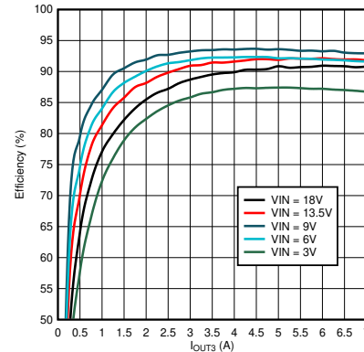
Figure 9-9. Efficiency vs. I_{OUT3} (FPWM)
