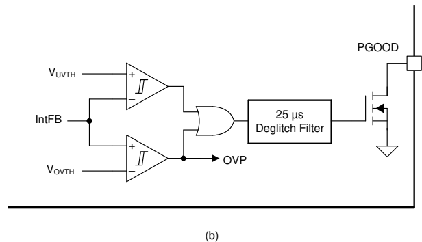
Figure 8-6. Power Good Monitor (b) Buck configuration
