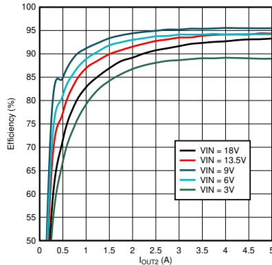
Figure 9-8. Efficiency vs. I_{OUT2} (FPWM)
