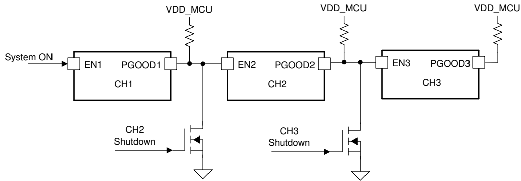
Figure 9-6. Sequential Start-up
