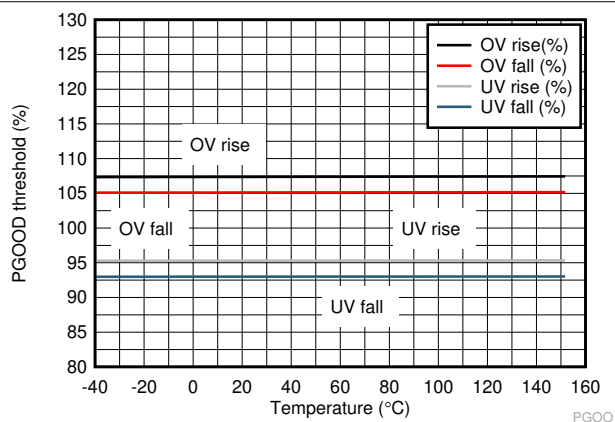
Figure 7-5. PGOOD Threshold ( V_{OVTH} , V_{UVTH} ) vs Temperature
