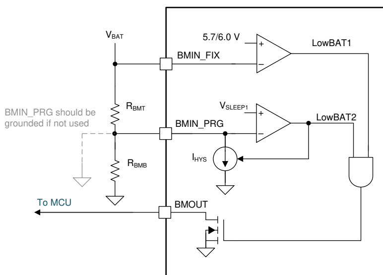
Figure 8-25. Battery Monitor
