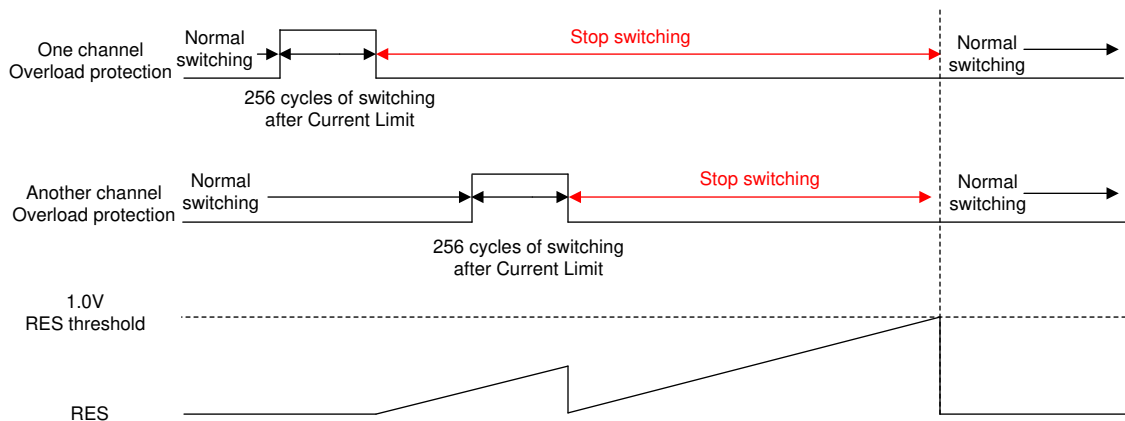
Figure 8-21. Hiccup Mode Overload Protection (Multiple Channel Faults)
