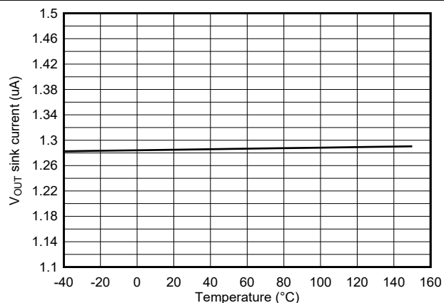
Figure 7-15. V_{OUT} Sink Current vs Temperature (Deep Sleep)
