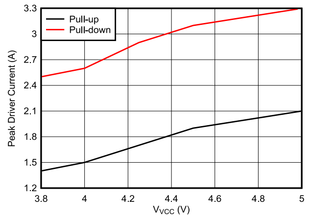
Figure 7-10. V VCC vs Peak Driver Current
