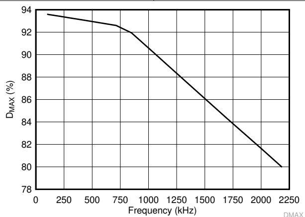
Figure 7-17. D_{MAX} vs Frequency
