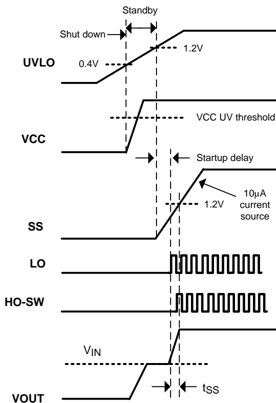
Figure 22. Startup Sequence
