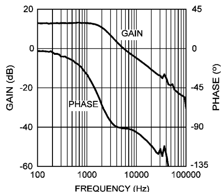
Figure 7-3. Modulator Gain and Phase
