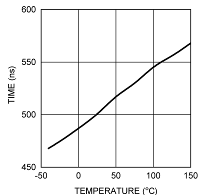
Figure 5-11. Forced HO Off-time vs Temperature VCCX = 5 V
