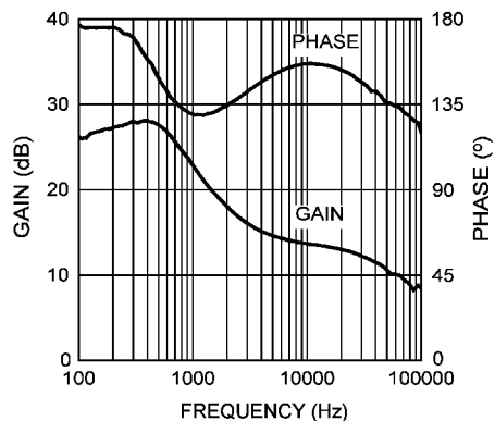
Figure 7-4. Error Amplifier Gain and Phase
