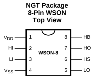
Pin Functions
