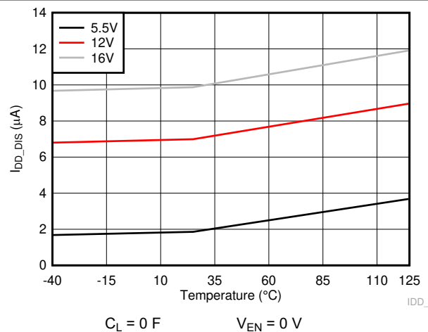
Figure 6-6. VDD Current When Disabled
