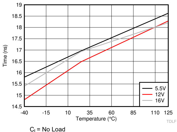
Figure 6-23. LO Falling Propagation Delay (TDLFF)
