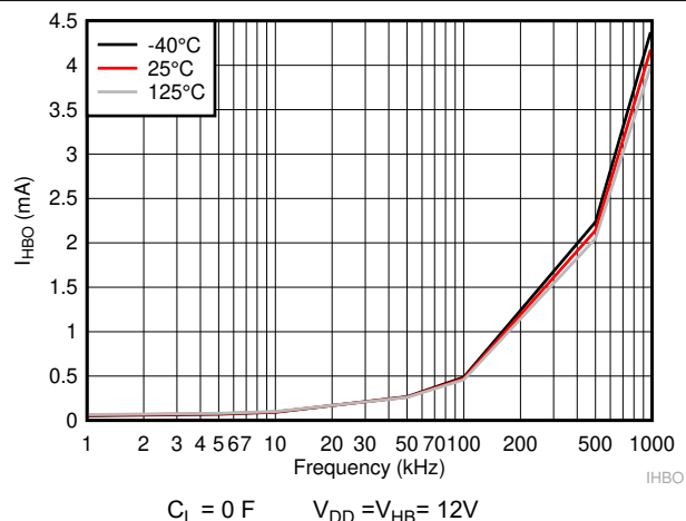
Figure 6-5. HB Operating Current
