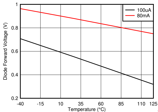
Figure 6-14. Boot Diode Forward Voltage Drop
