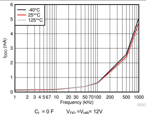
Figure 6-4. VDD Operating Current
