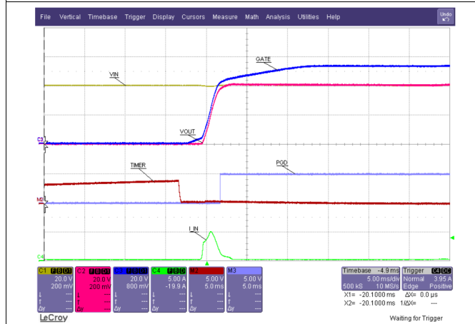
Figure 28. Insertion Delay
