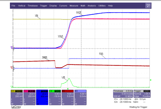
Figure 29. Start-Up
