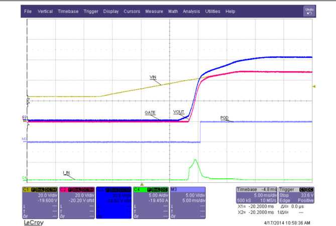
Figure 33. Under-Voltage
