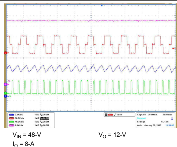
Figure 8-14. Steady State Operation Waveform
