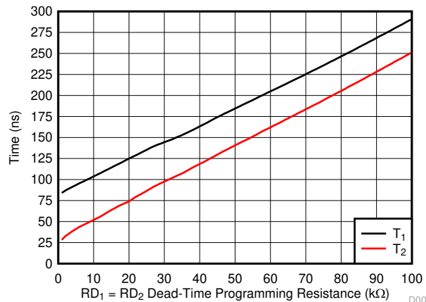
Figure 6-7. Dead Time vs Programming Resistance
