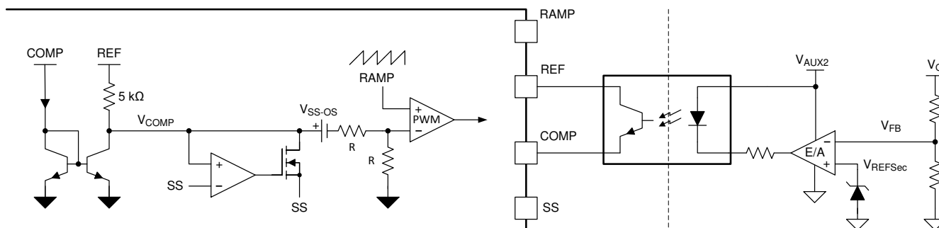
Figure 7-2. Voltage-Mode Feedback Control Loop for Half-Bridge Converter
