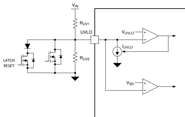
Figure 8-6. Latch Reset
