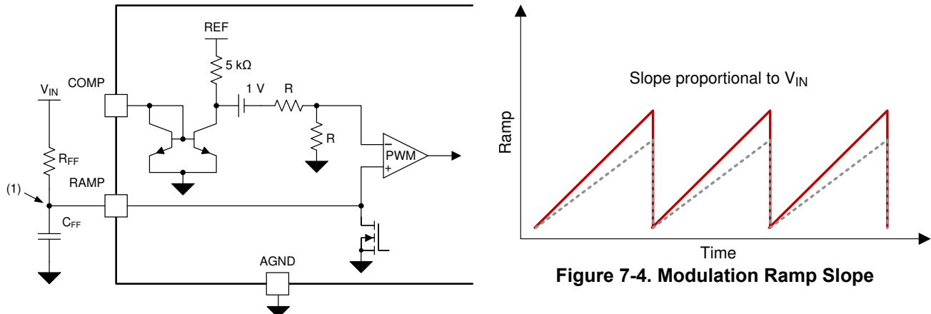
A. Slope proportional to input voltage (see Figure 7-4)
