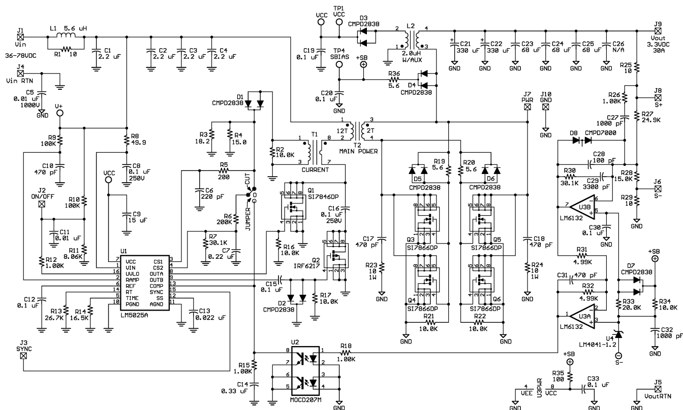
Figure 22. Application Circuit
