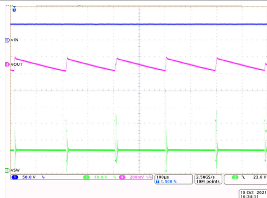
Figure 9-9. Light-Load Switching
